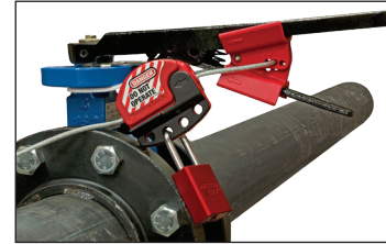
S3920 device acts as a wedge between the two handles; locked out with S806 adjustable cable & padlock.
