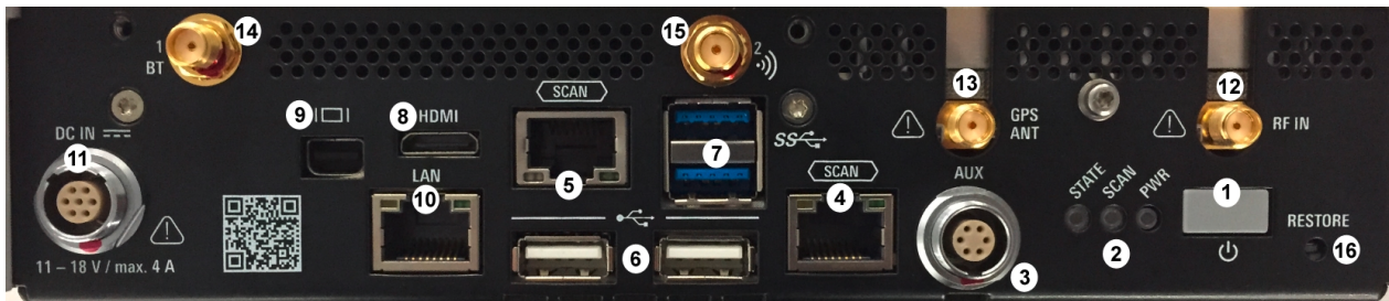
Figure 4-2: R&S TSMA - Rear Panel
