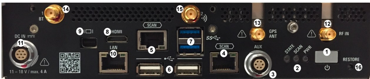
Figure 5-2: R&S TSMA - Rear Panel
