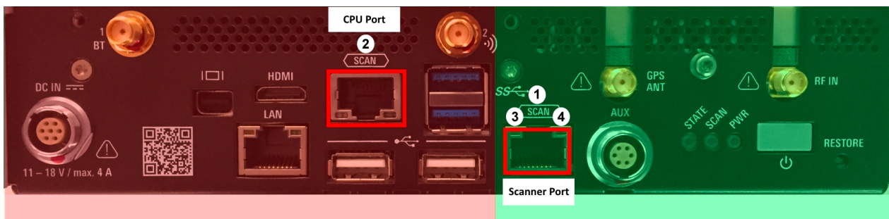
Figure 5-3: Connectors of the R&S TSMA
