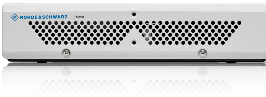
Figure 5-1: R&S TSMA - Front Panel
