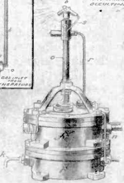
6 THE FLASHING APPARATUS AN INGENUOUS SELF-ACTING VALVE OPERATED BY GAS PRESSURE AND FURNISHING ANY CHARACTER OF OCCULTING LIGHT.
