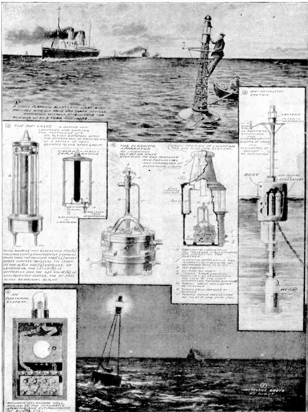
TWO TYPES OF ACETYLENE BUOYS PROPOSED TO MARK THE ENTRANCE TO THE PANAMA CANAL. BOTH ARE CONTROLLED BY THE LIGHT OF THE SUN—ONE BY AN ELECTRICAL DEVICE EMBODYING THE SELENIUM CELL
