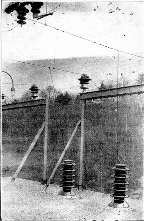
HIGH TENSION ROOF WIRING
