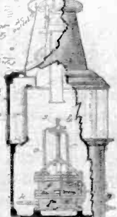
7 CROSS SECTION OF LANTERN FOR THE FLASHING SYSTEM.
