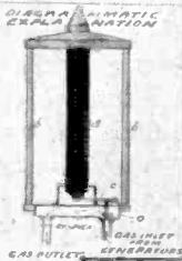
5 THE SUN VALVE A DEVICE FOR LOCKING AND RARIFYING THE ACETYLENE MIXTURE. ITS ACTION DEPENDS UPON THE DIFFERENCE IN EXPANSION OF A SERIES OF RODS EXPOSED TO THE SAME LIGHT.
