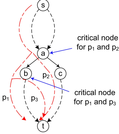
Figure 7. Critical nodes for pairs of paths.
