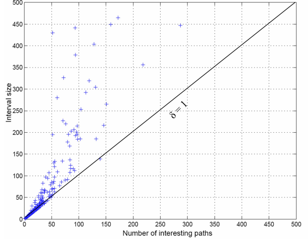
Figure 16. \delta values achieved by preferential path profiling.
