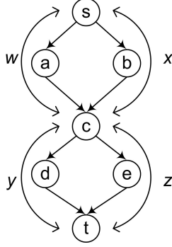
Figure 5. A counterexample for separation of paths.
