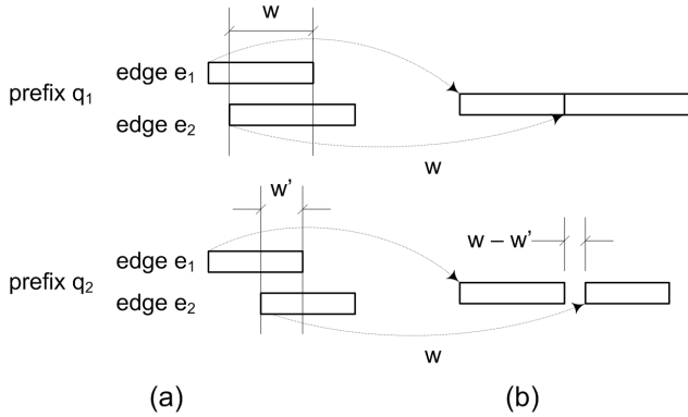
Figure 9. The effect of using the join operator to conservatively assign weights to edges. (a) Intervals induced by the prefixes before the join, and (b) effective intervals after the join.
