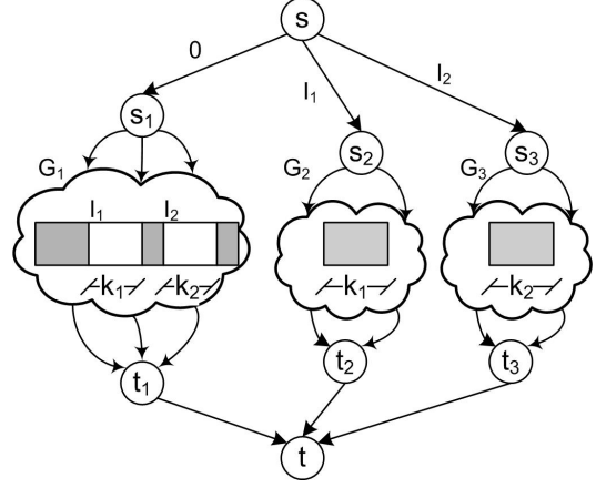
Figure 11. Figure illustrating a scenario in which PPP assigns a sub-optimal numbering but an optimal numbering clearly exists.
