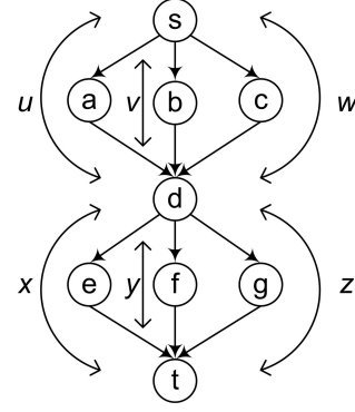
Figure 6. A counterexample for perfect edge assignment.
