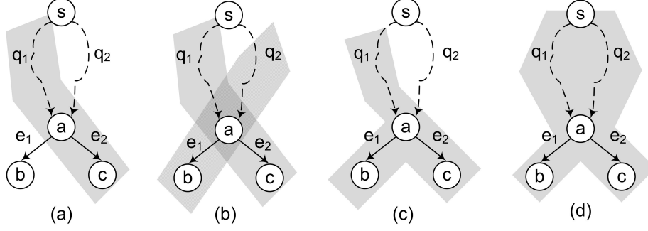
Figure 8. The assignment of weights to edges under four scenarios
