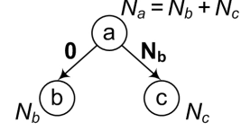
Figure 2. Assignment of weights to edges using the Ball-Larus algorithm
