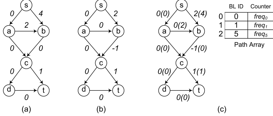
Figure 3. Motivating example for PPP. (a) A DAG G with 6 paths with edges numbered using the Ball-Larus algorithm. (b) G with edges having only PPP assigned numbers for three interesting paths I = \{sacdt, sact, sbct\} . (c) G with edges assigned two numbers, a PPP number and a Ball-Larus number (in parenthesis). The path array is accessed using the PPP counter.
