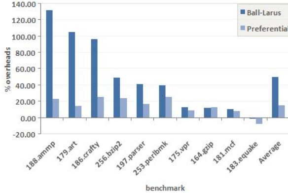
Figure 15. Overheads of preferential path profiling.
