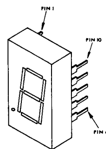
HP5082-7623
