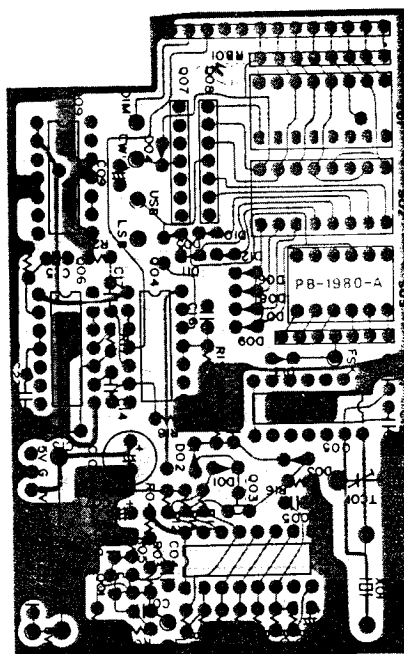
Viewed from solder side
