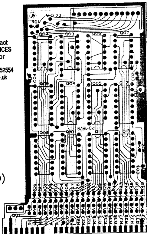
Viewed from solder side
