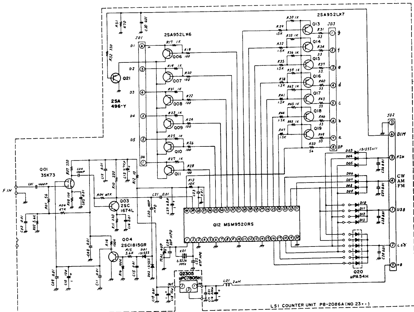
DISPLAY/COUNTER UNIT
