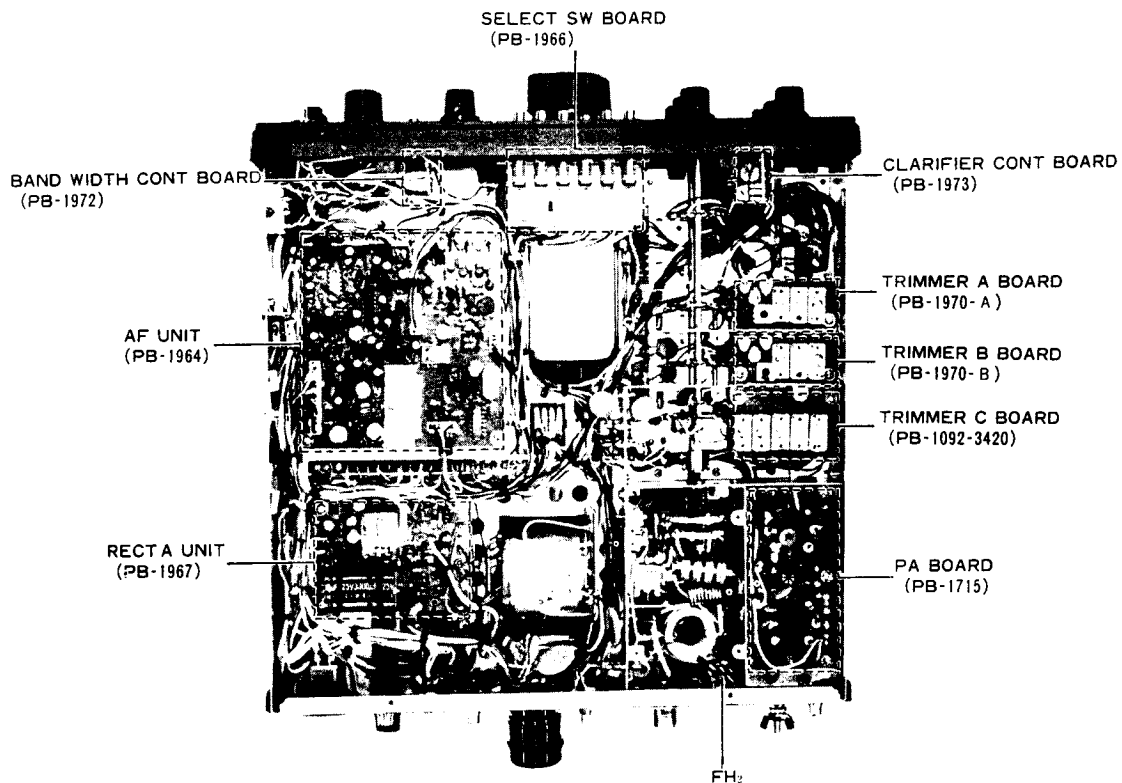
BOTTOM VIEW
