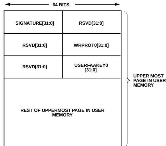
Figure 11. Uppermost Page of User Flash 0
