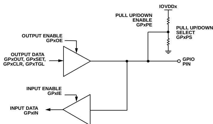
Figure 25. GPIO Block diagram
