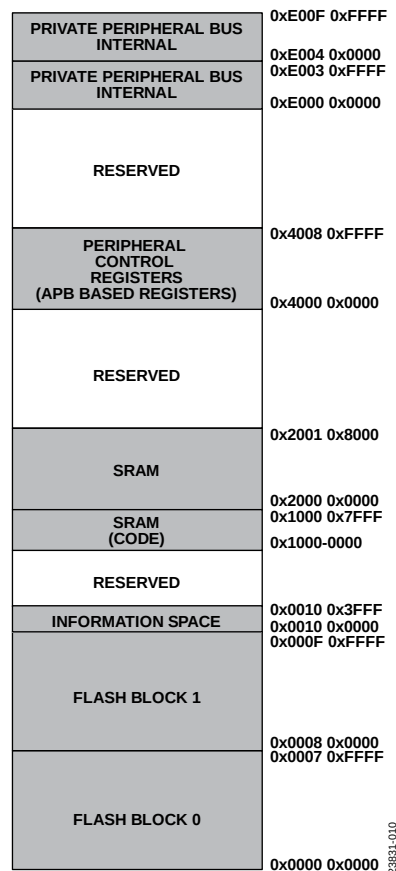
Figure 9. ADuCM410 and ADuCM420 Memory Map (Default)
