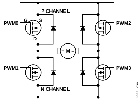
Figure 38. Example H Bridge Configuration
