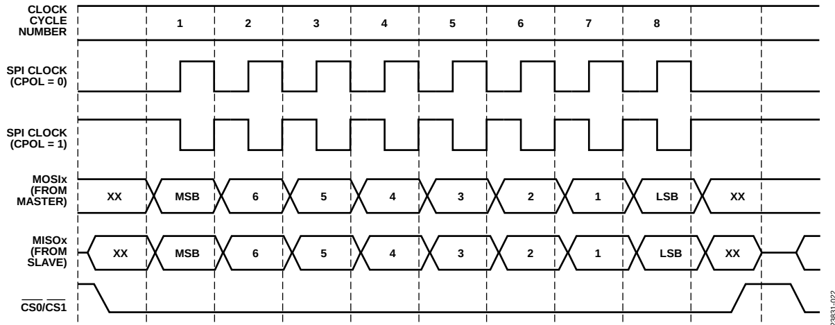
Figure 20. SPI Transfer Protocol, CPHA = 0
