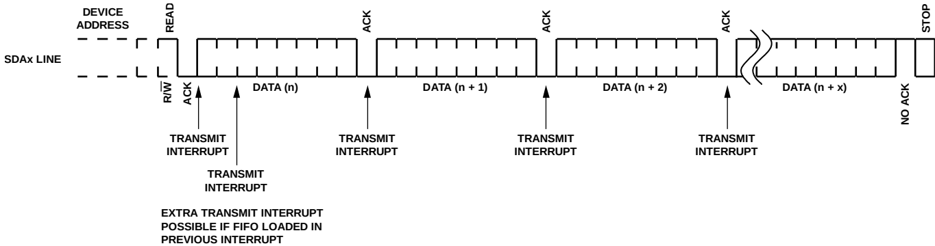
Figure 19. I²C Slave Transmit Interrupt Details
