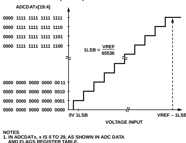
Figure 4. ADC Transfer Function: Single-Ended Mode
