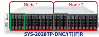
SYS-2028TP-DNC/(T)(F)R Up to 4x NVMe + 8x SAS 3.0 drives (per node)
