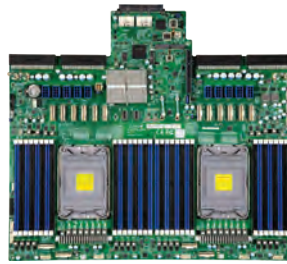
GPU Serverboard
