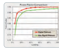
Power Factor Comparison
