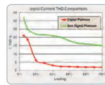
Input Current THD Comparison
