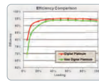
Efficiency Comparison
