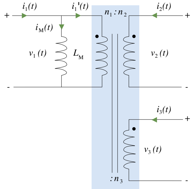
Figure 18. Multi winding magnetic element.
