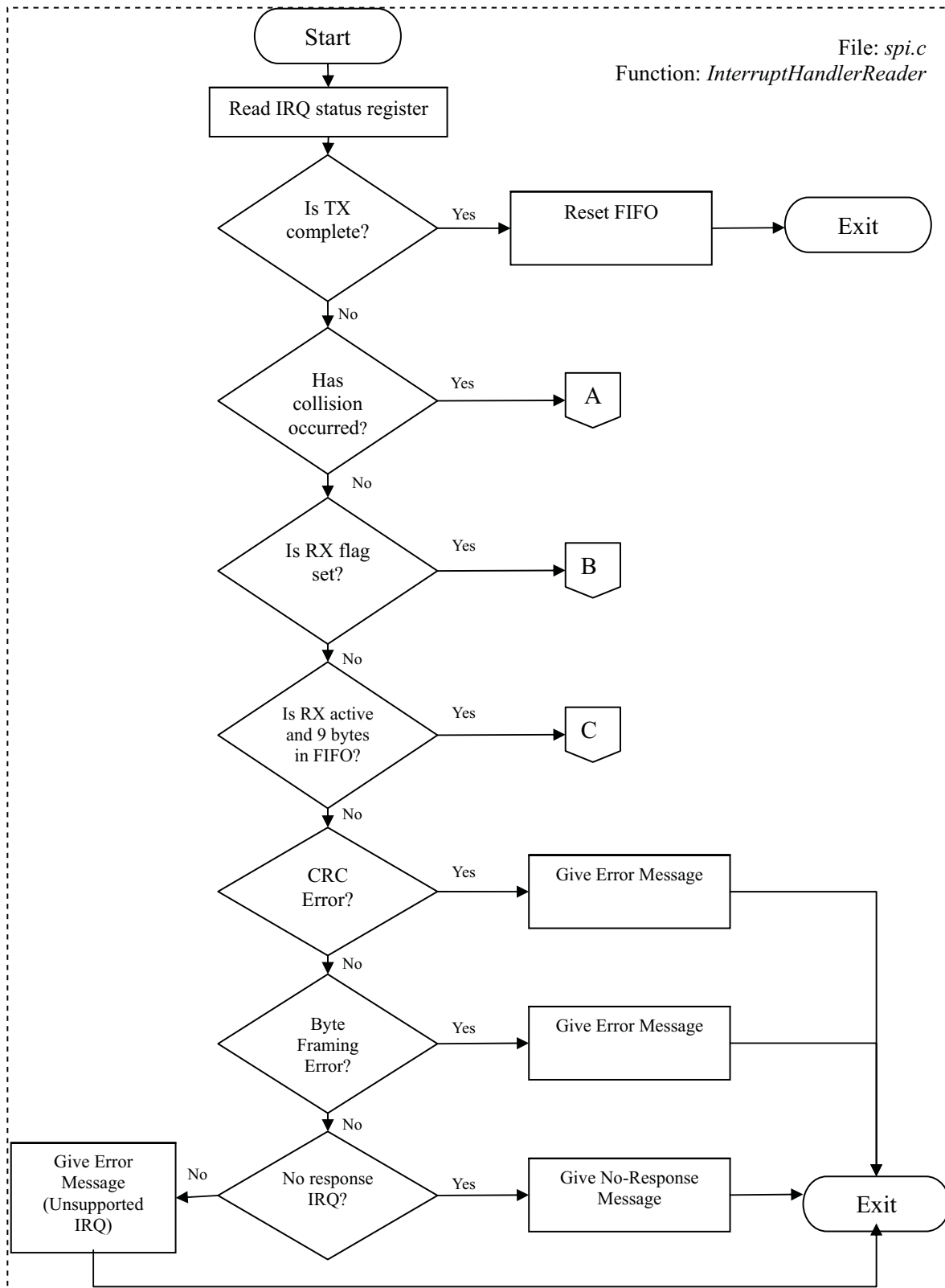
Figure 3. Interrupt Handler Routine (1)
