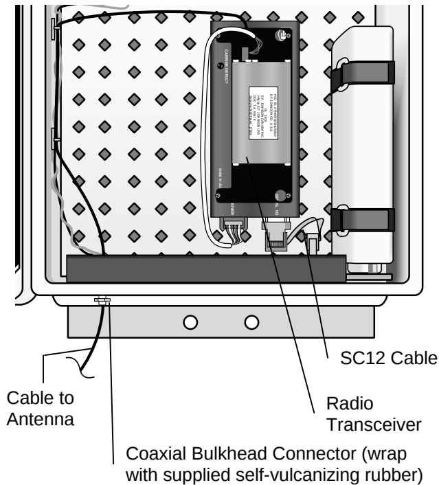
FIGURE 3.3-5. RF95 RF Modem and RF100/RF200 Transceiver
