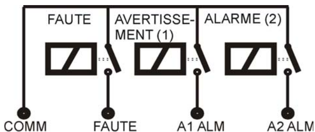
Figure 3-E Sorties relais
