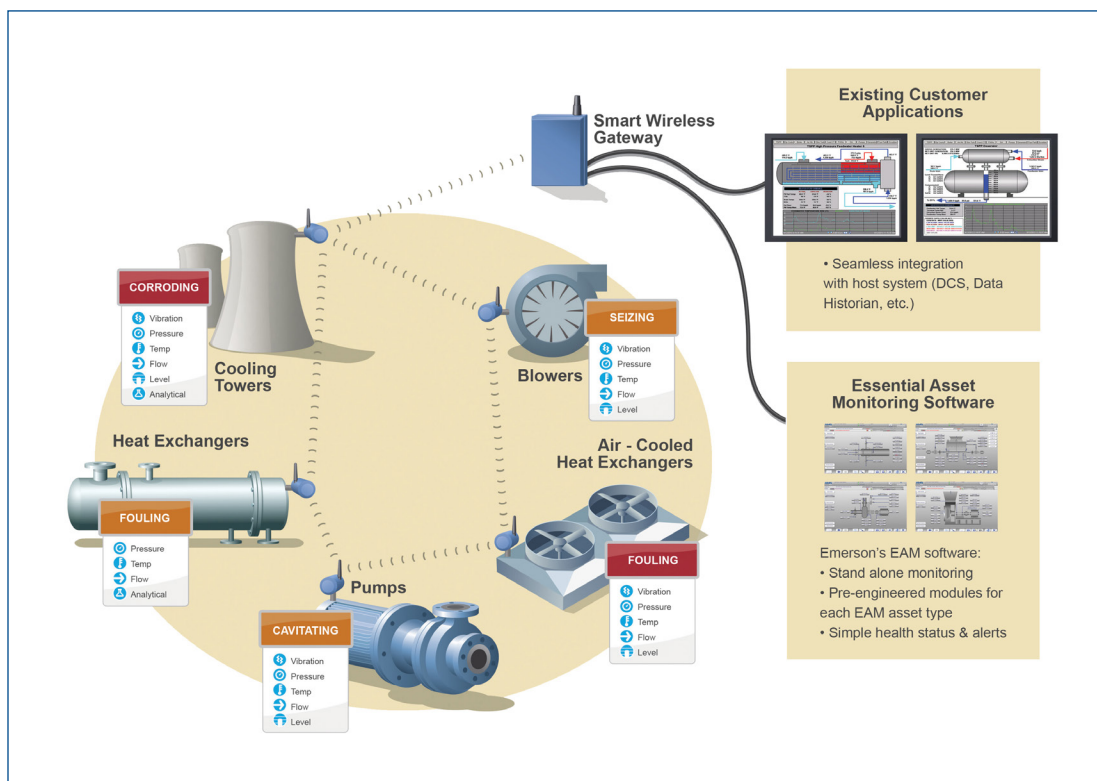
Figure 2 — Essential Asset Monitoring provides visibility of abnormal situations, enabling avoidance of process interruptions.
