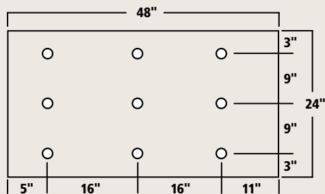
Pattern B 16" O.C. stud fastening pattern. Note: For pattern "B" stud fastening over non-screwable sheathing, fastener spacing does not exceed 16". O.C. variable not to exceed 11".
