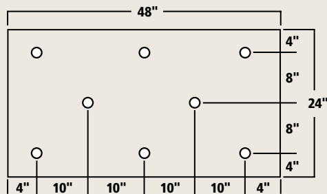
Pattern C Wood sheathing, masonry and some metal sidings.
