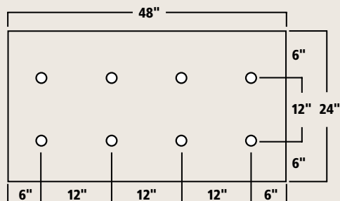
Pattern A Wood sheathing, masonry and some metal sidings.
