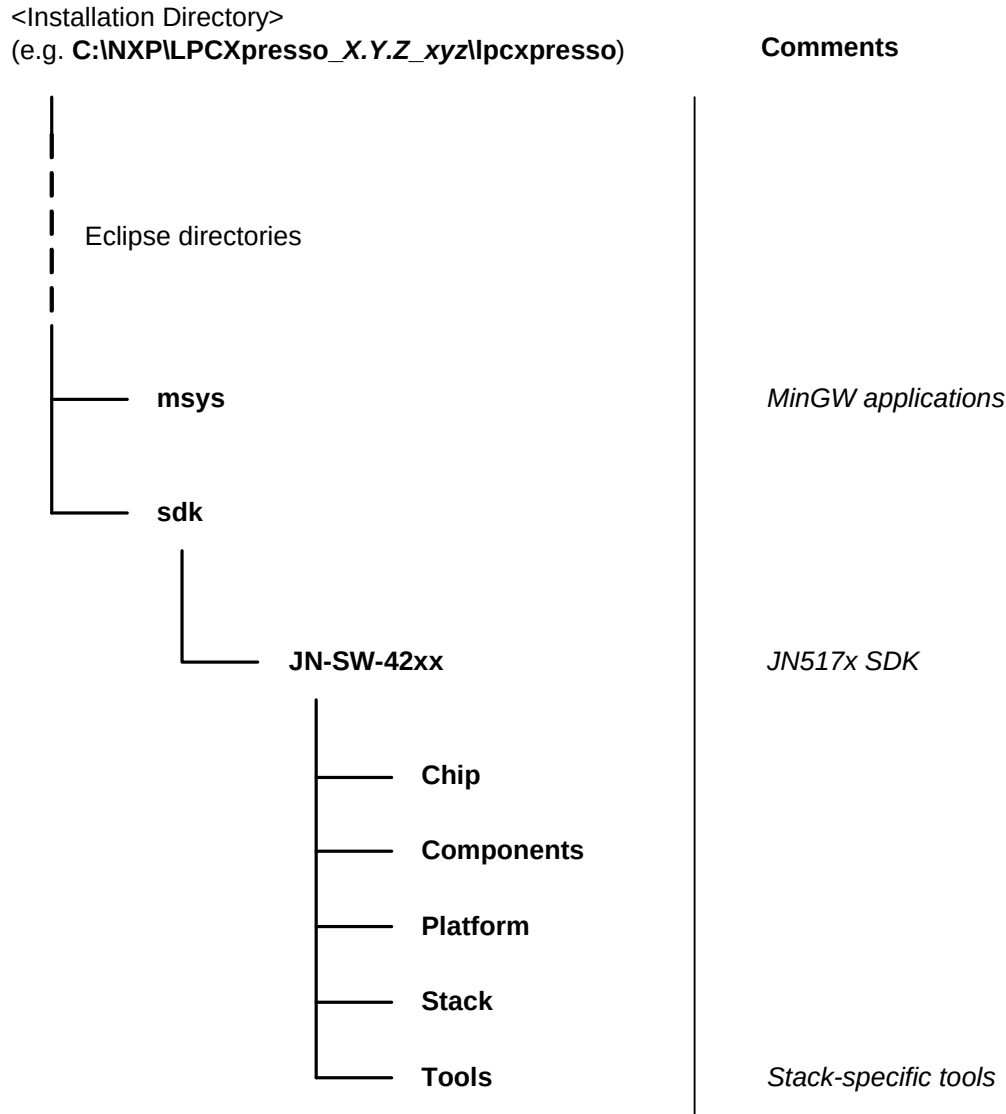
Figure 1: Directory Structure
