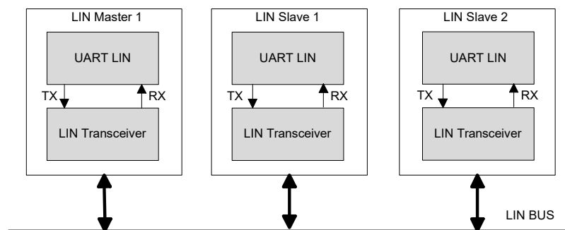
Figure 14-14. UART_LIN and LIN Transceiver
