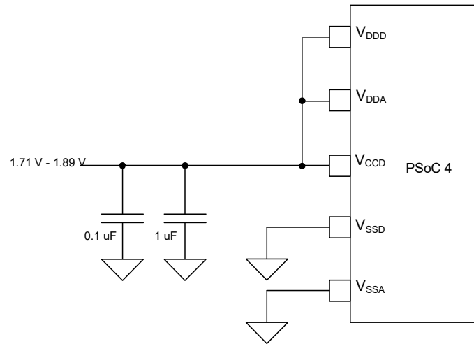
Figure 8-3. Single Unregulated V_{DDD} Supply
