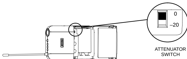
THE UC1 TRANSMITTER ATTENUATION SWITCH
