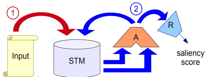
Figure 12 – The short-term memory (STM) holds a collection of representation vectors. The two possible actions are (1) inserting a new representation vector into the STM, and (2) replacing two vectors from the STM by the output of the association module.
