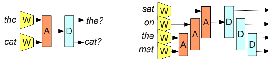
Figure 10 – Navigating intermediate representations with the dissociation module.
