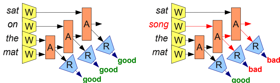
Figure 8 – Unsupervised training (see text.)
