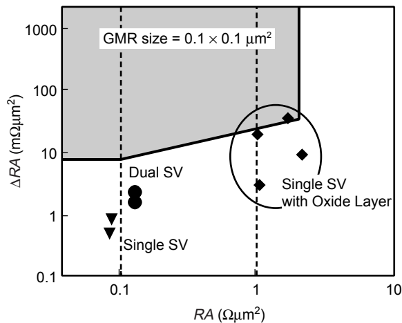
Figure 8 \Delta RA vs. RA of SV films.
