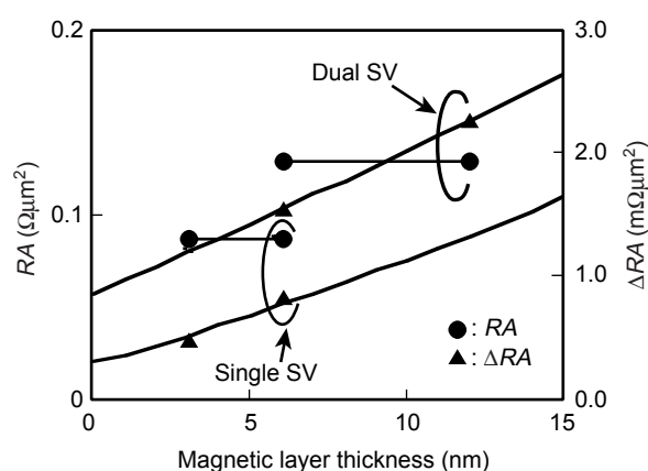
Figure 6 Total magnetic layer thickness dependence of RA and \Delta RA . Solid lines are fitted to the two-current series resistor model.
