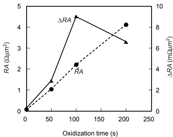
Figure 7 RA and \Delta RA of a single SV with an oxide layer.
