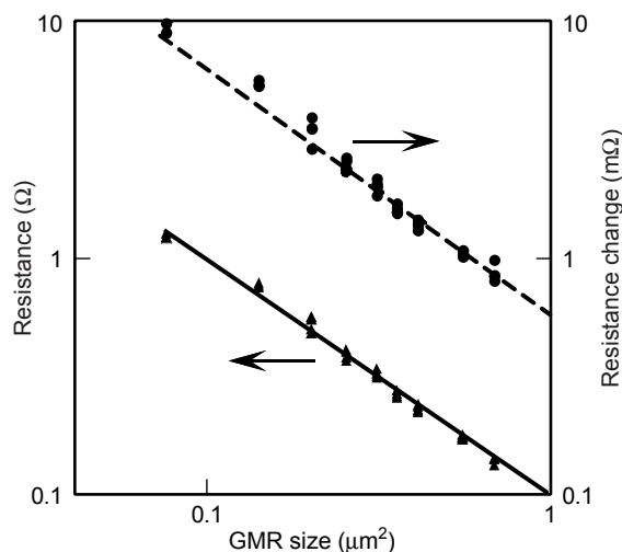
Figure 5 Resistance R and resistance change \Delta R of the element as a function of GMR size A . Solid and dashed lines are the fitting lines for R = 0.1/A ( \Omega ) and \Delta R = 0.59/A (m \Omega ).
