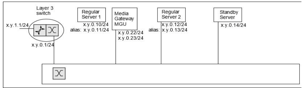
Figure 3: Server redundancy without network redundancy
