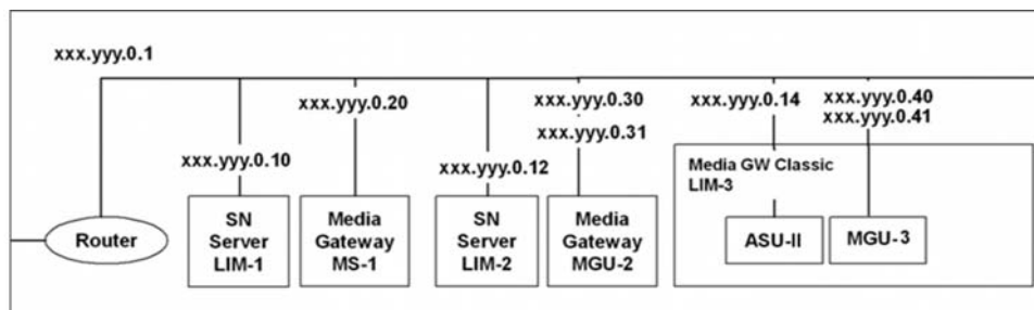
Figure 1: A non-redundant scenario with MGU and MS media gateways
