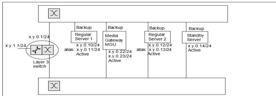
Figure 2: Server redundancy with Ethernet bonded network redundancy. System database is not shown here.
