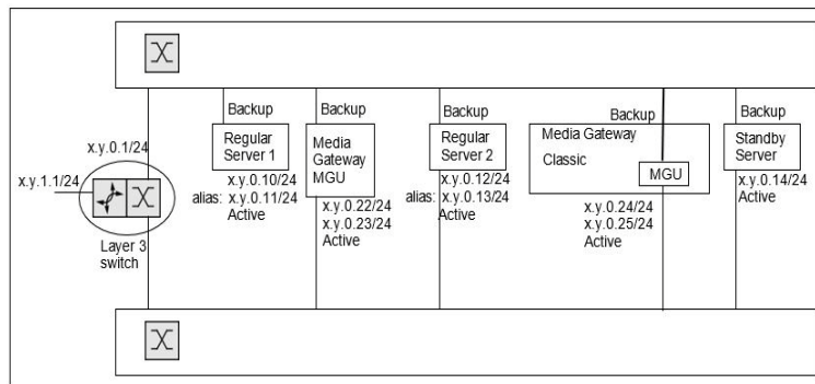
Figure 4: Server redundancy with Ethernet bonded network redundancy
