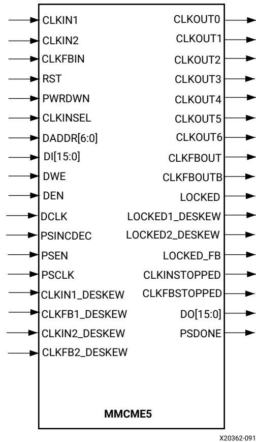
Figure 29: MMCMES Primitive
