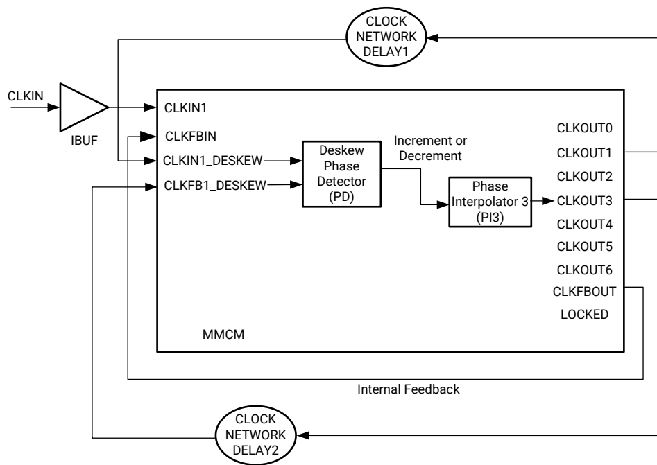
Figure 30: MMCM Clock Network Deskew Using Deskew Logic
