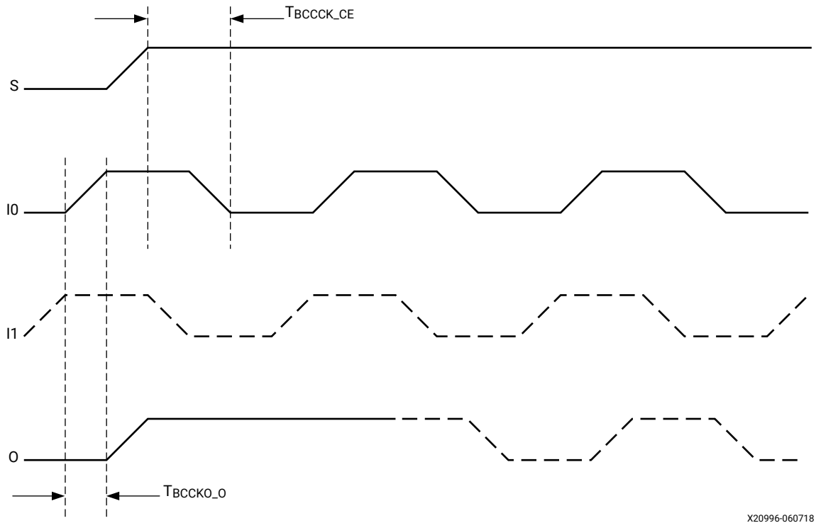
Figure 12: BUFGMUX_1 Timing Diagram
