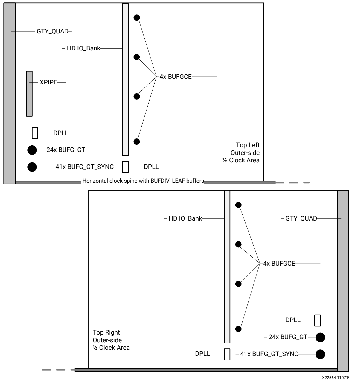
Figure 25: Top Left and Right Clock Regions
