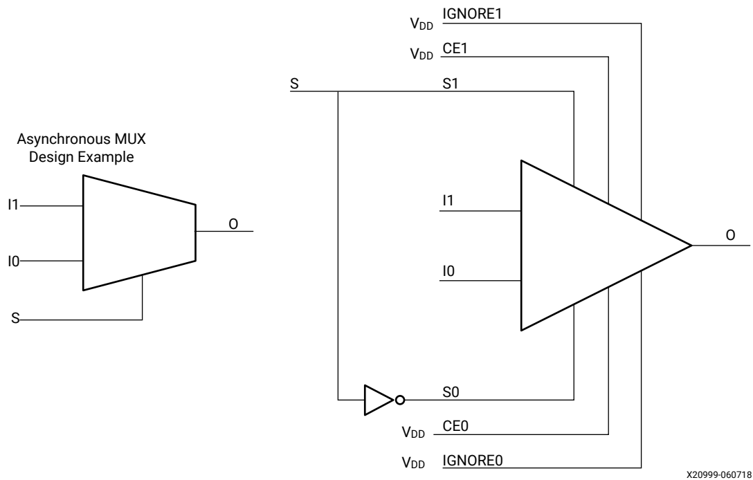
Figure 15: Asynchronous MUX using BUFCTRL Design Example
