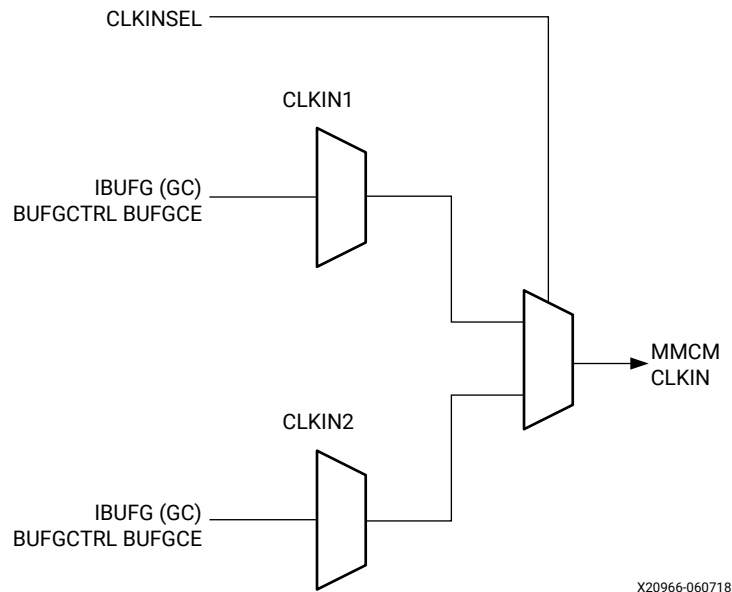
Figure 35: Input Clock Switching
