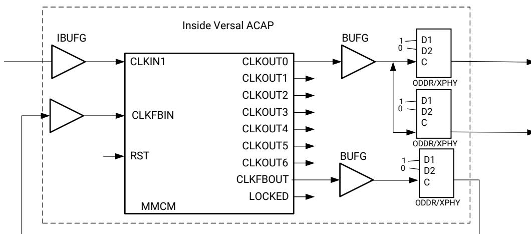
Figure 38: Zero Delay Buffer - CLKFBOUT Deskew
