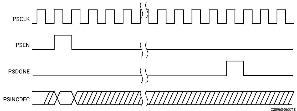
Figure 31: Phase Shift Timing Diagram
