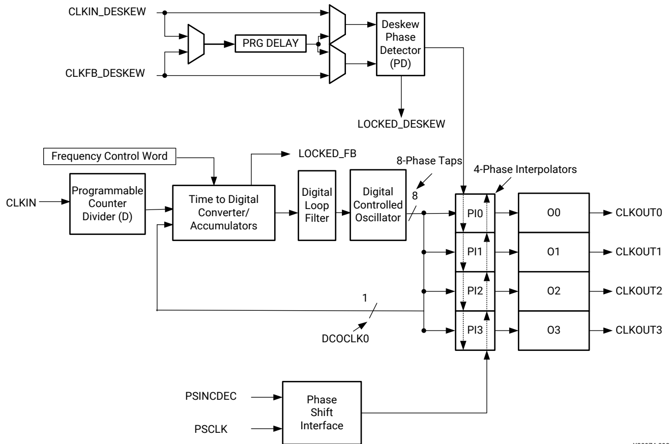
Figure 48: DPLL Block Diagram
