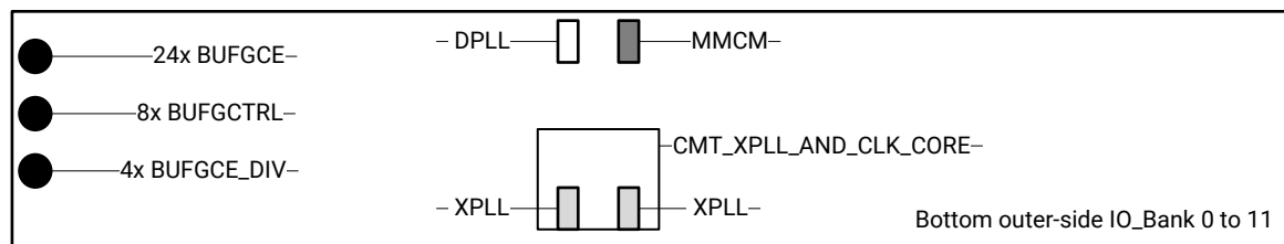
Figure 27: Bottom Clock Regions
