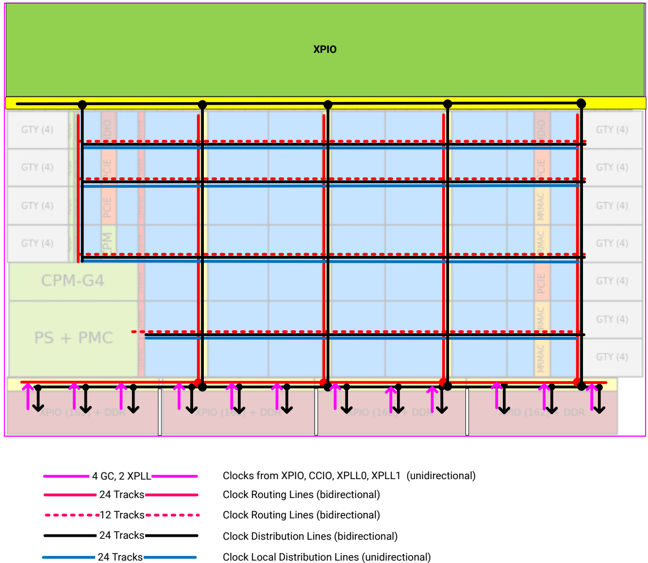
Figure 3: Clock Routing Architecture
