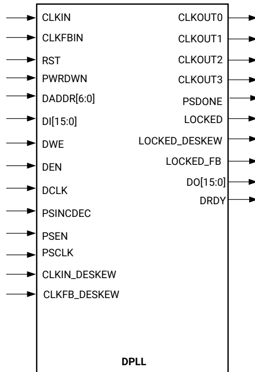
Figure 49: DPLL Primitive
