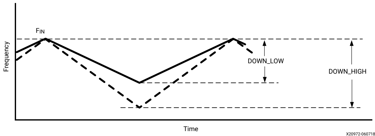
Figure 46: Down-Spread Modulation
