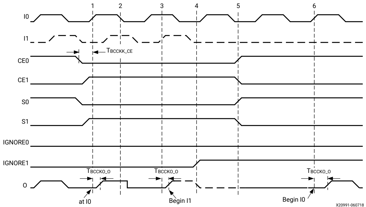
Figure 7: BUFGCTRL Timing Diagram
