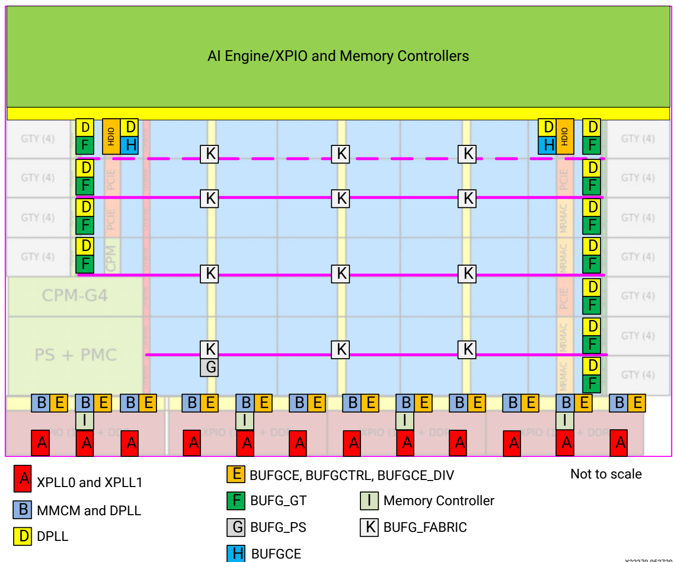
Figure 2: Locations of Clock Buffer Resources and Clock Management Functions
