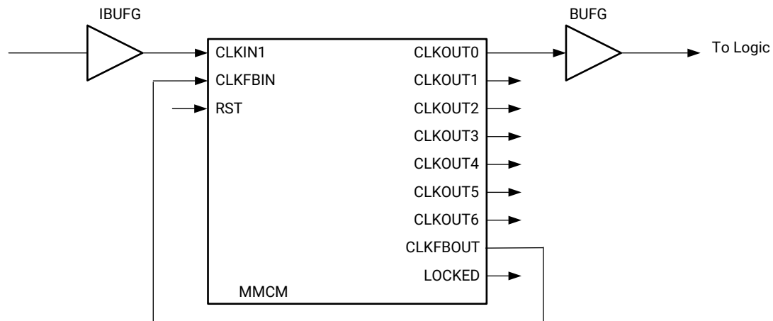
Figure 37: MMCM with Internal Feedback - No Deskew
