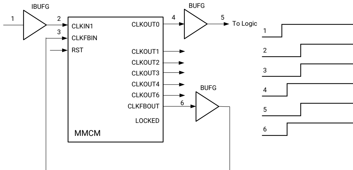
Figure 36: Global Clock Network Deskew Using Two BUFGs
