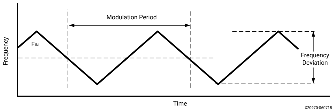
Figure 44: Center-Spread Modulation
