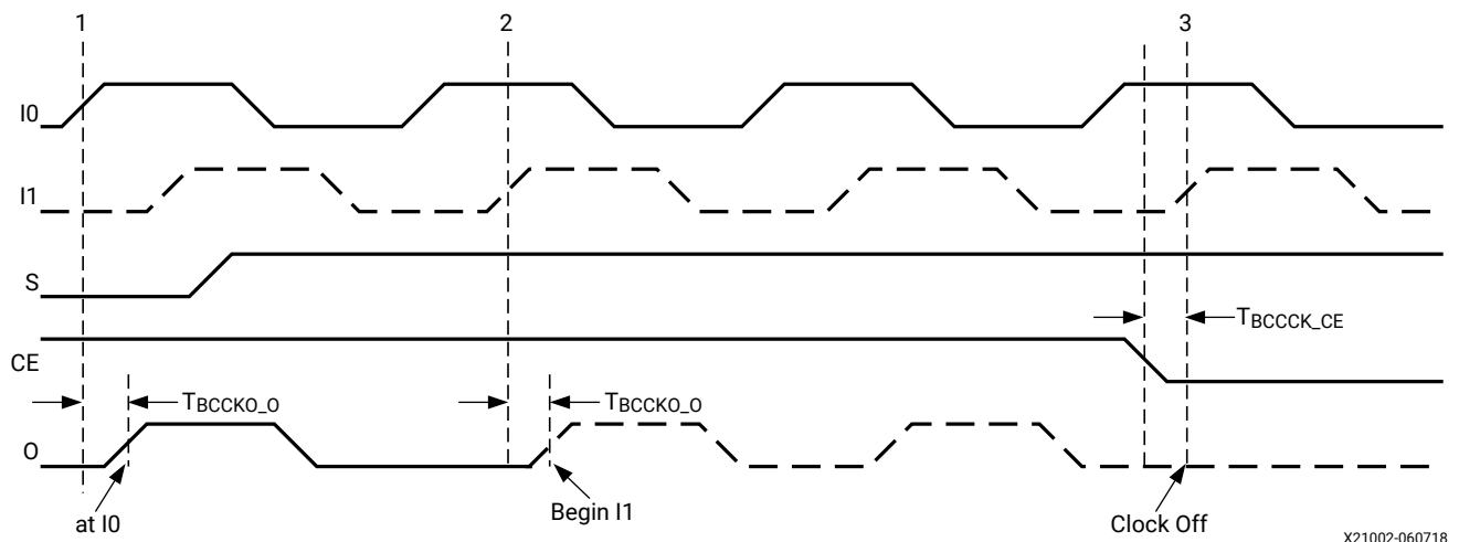
Figure 18: BUFGMUX_CTRL with a CE Timing Diagram
