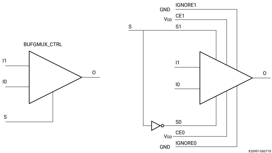
Figure 13: BUFGMUX_CTRL using BUFGCTRL
