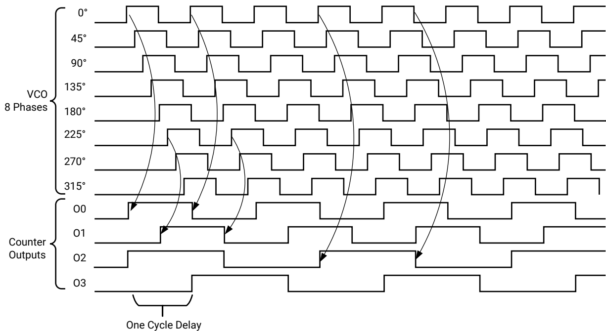
Figure 34: Selecting VCO Phases
