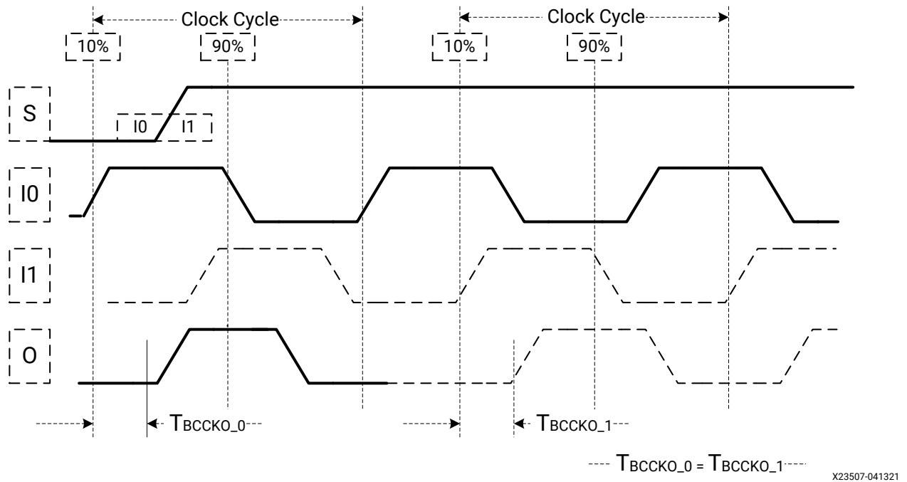
Figure 14: BUFGMUX_CTRL Timing Diagram
