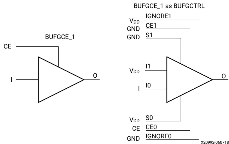
Figure 8: BUFGCE_1 using BUFGCTRL
