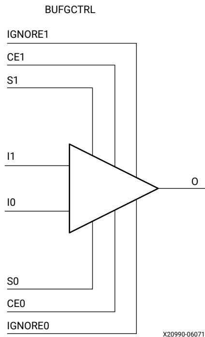
Figure 6: BUFGCTRL Primitive
