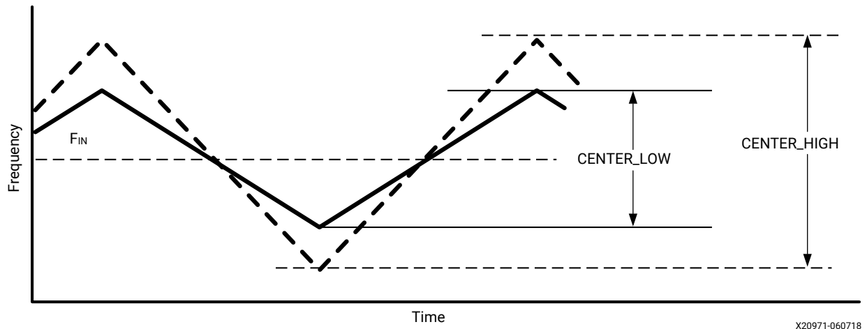
Figure 45: Center-Spread Modulation (CENTER_LOW vs. CENTER_HIGH)
