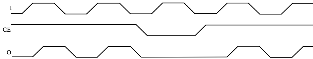
Figure 9: BUFGCE_1 Timing Diagram
