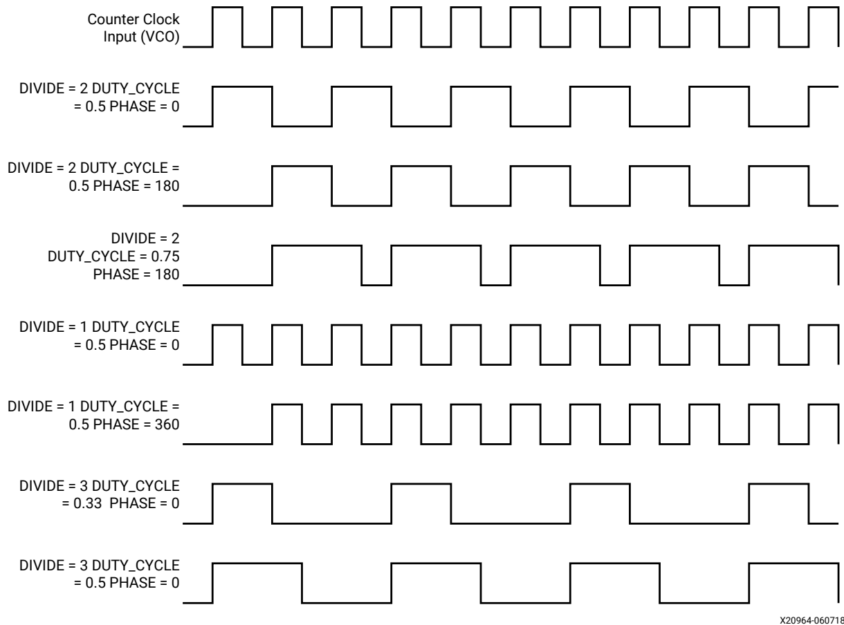
Figure 33: Output Counter Clock Synthesis Examples
