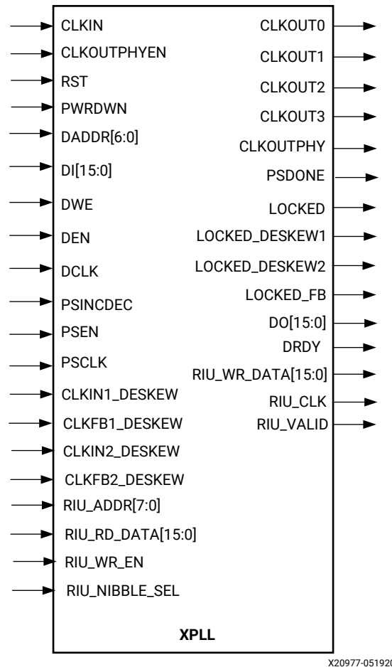
Figure 51: XPLL Primitive
