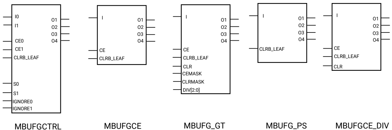
Figure 24: MBUFG Type Clock Buffers
