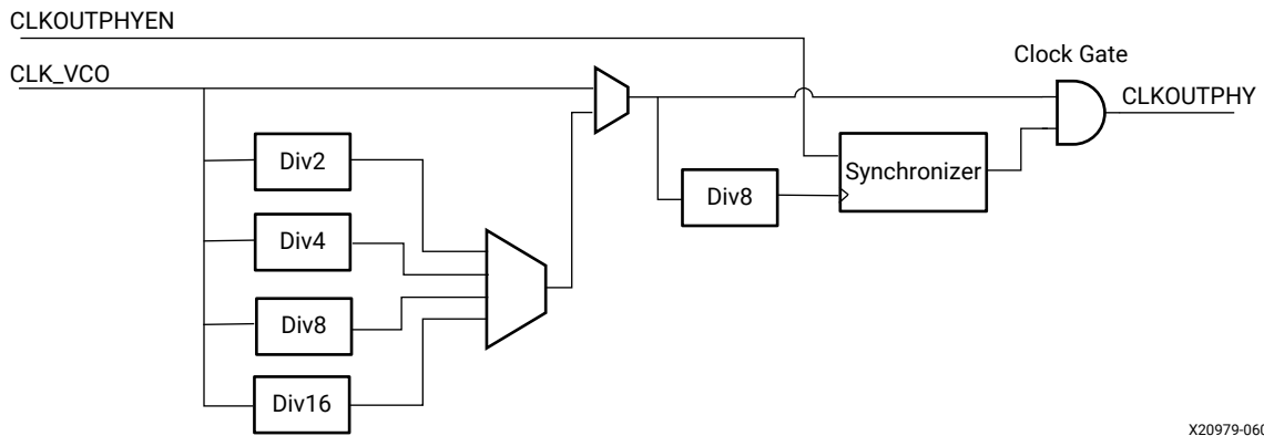
Figure 52: CLKOUTPHY Multiplexer Scheme
