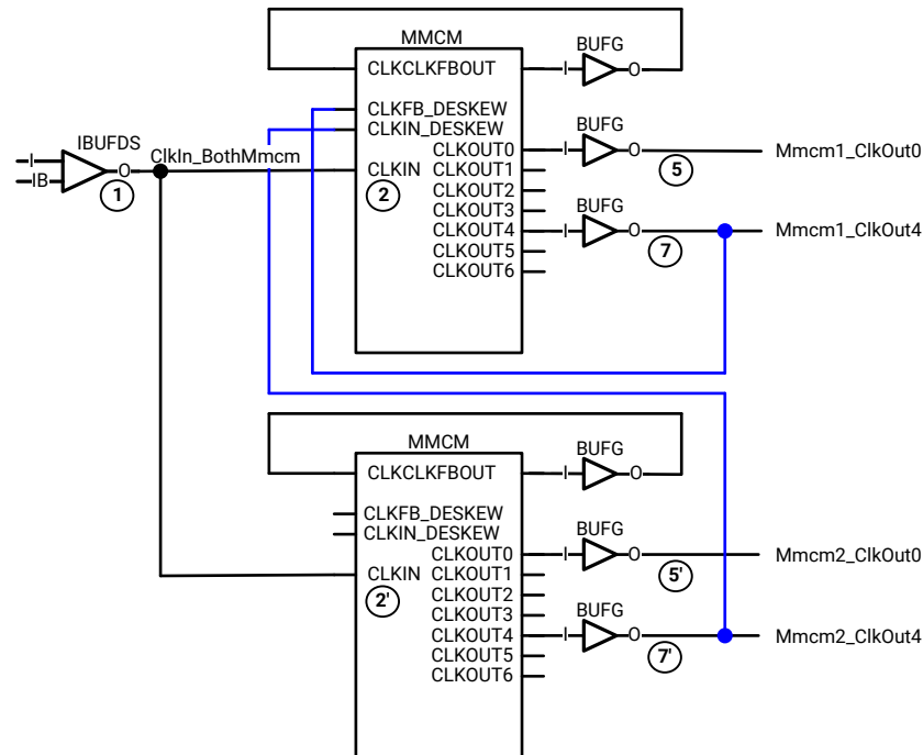
Figure 42: Dual MMCM Using DESKEW
