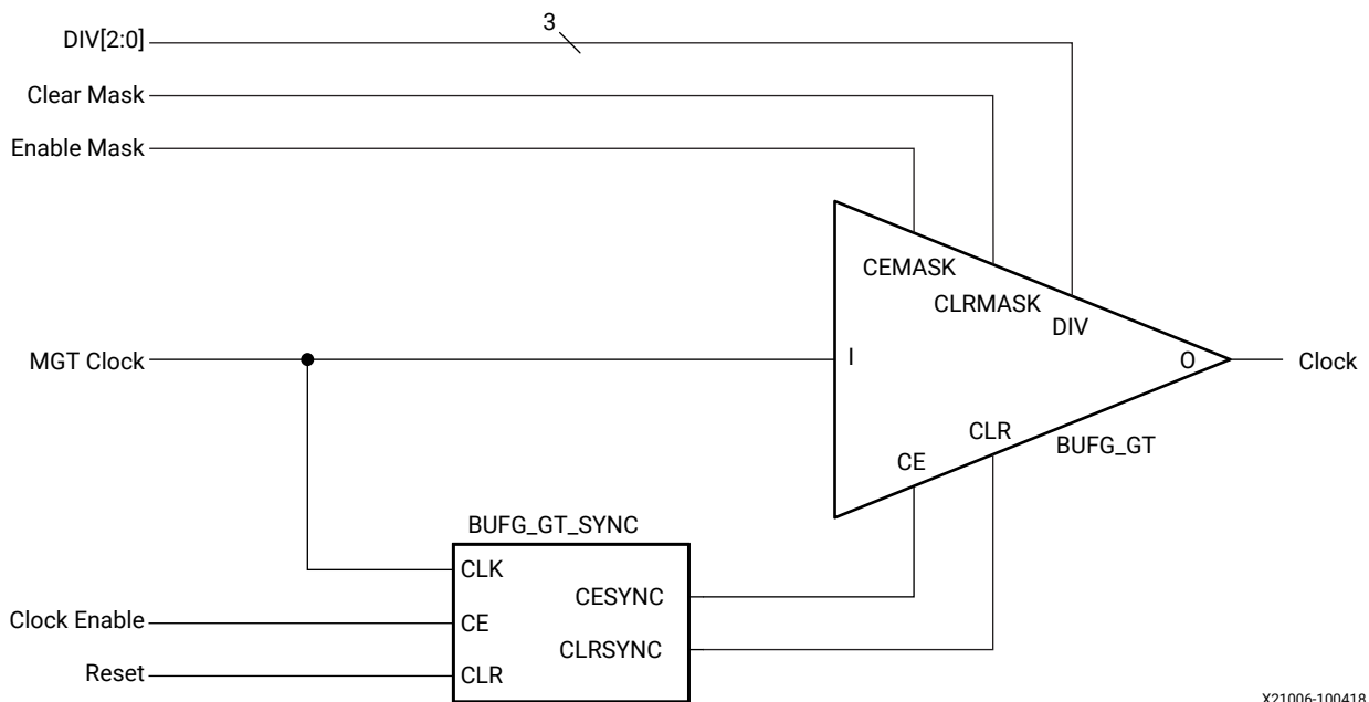
Figure 23: BUFG_GT Primitive
