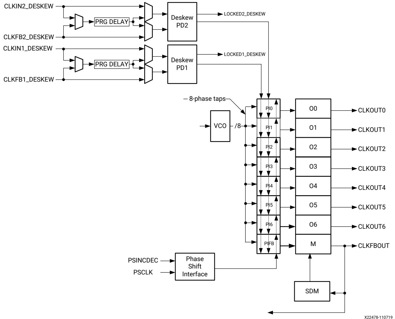
Figure 39: The Deskew Logic
