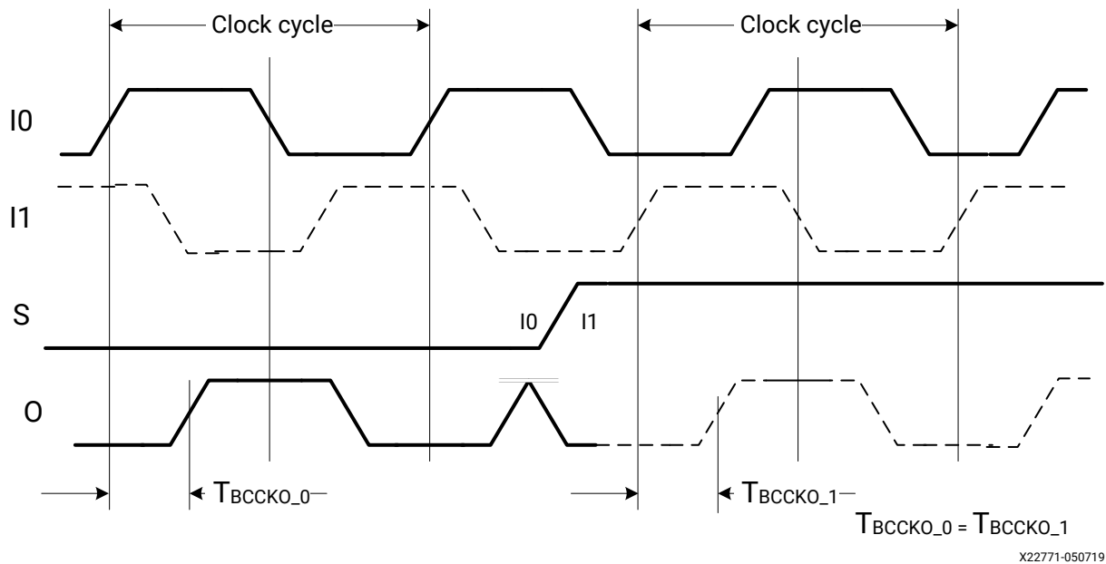
Figure 16: Asynchronous MUX Timing Diagram
