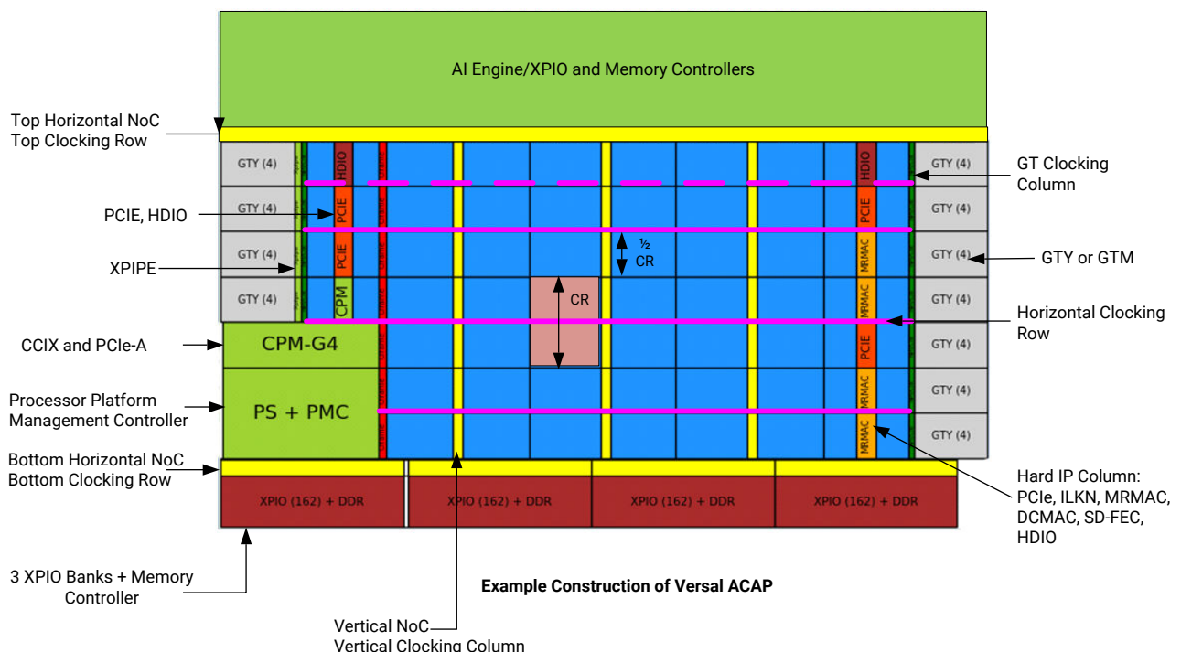
Figure 1: High-Level Architecture View
