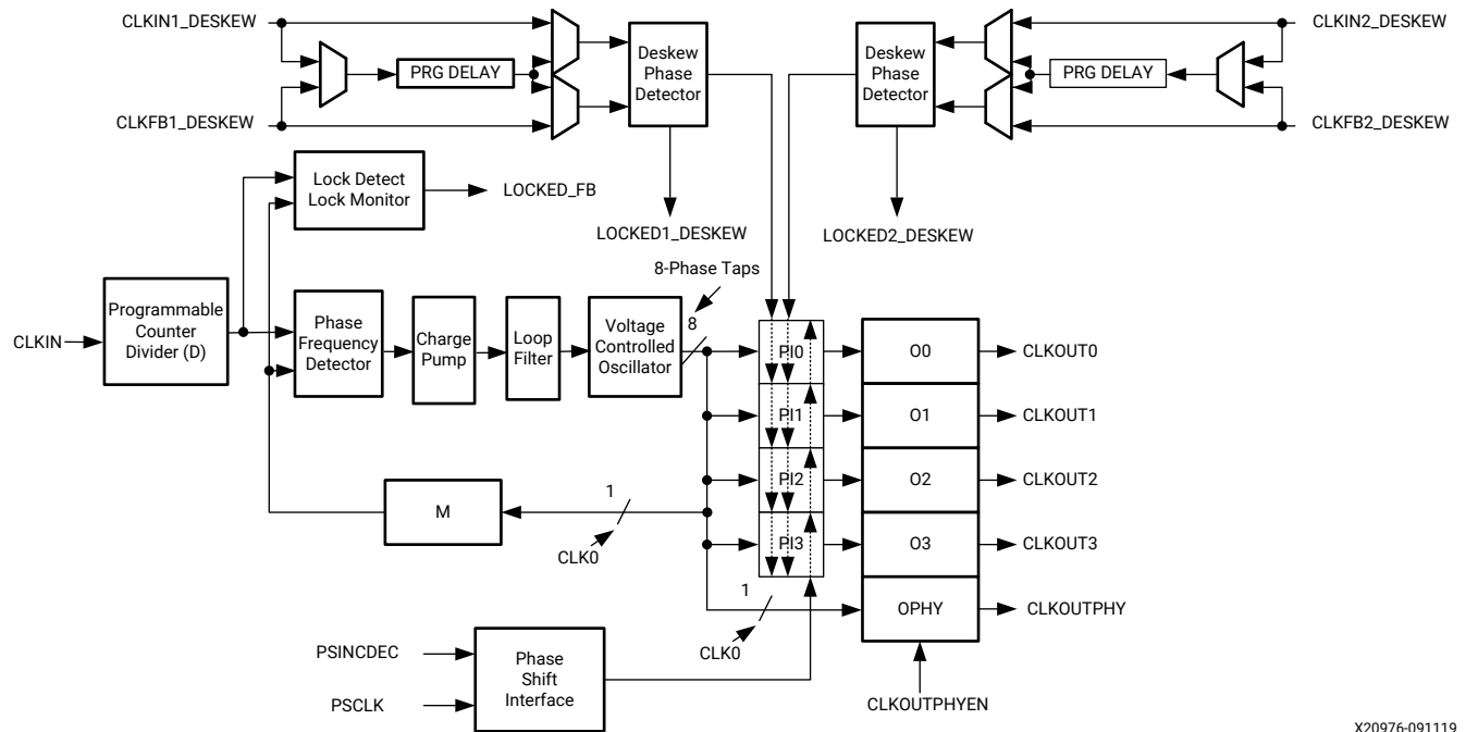
Figure 50: XPLL Block Diagram
