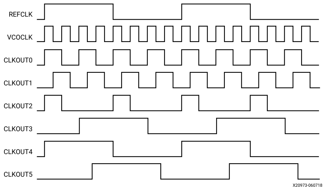
Figure 47: Example Waveform
