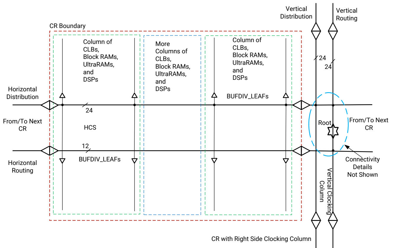
Figure 4: Clock Region
