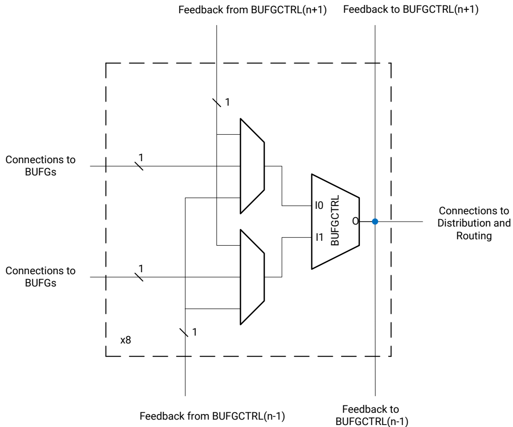
Figure 5: BUFGCTRL Cascading
