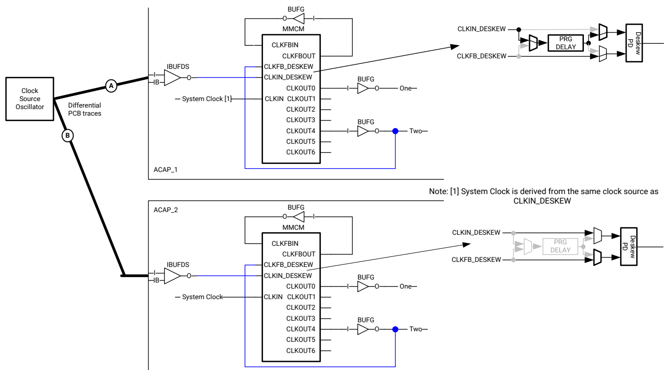
Figure 43: Deskew of External Versal ACAP Clocks - System Synchronous Design
