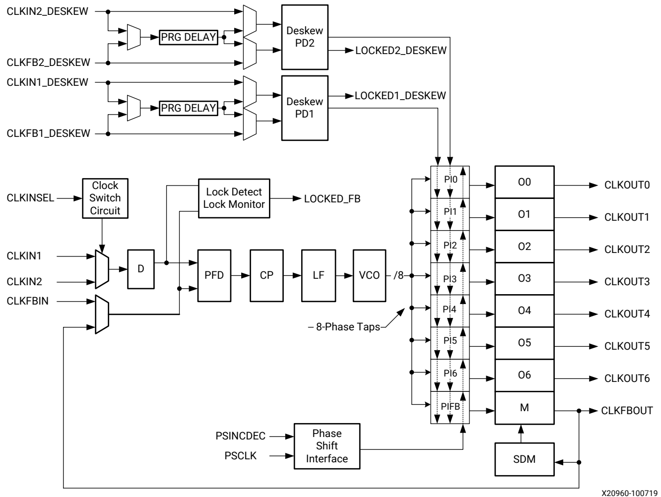
Figure 28: MMCM Block Diagram
