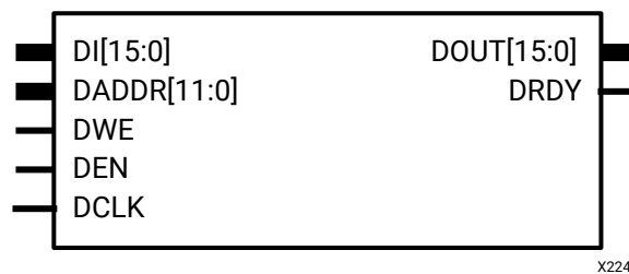
Figure 32: DRP Port
