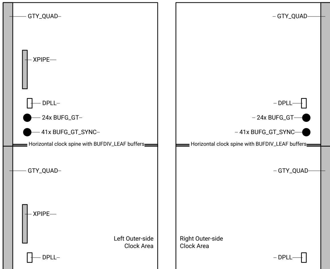
Figure 26: Middle Left and Right Clock Regions
