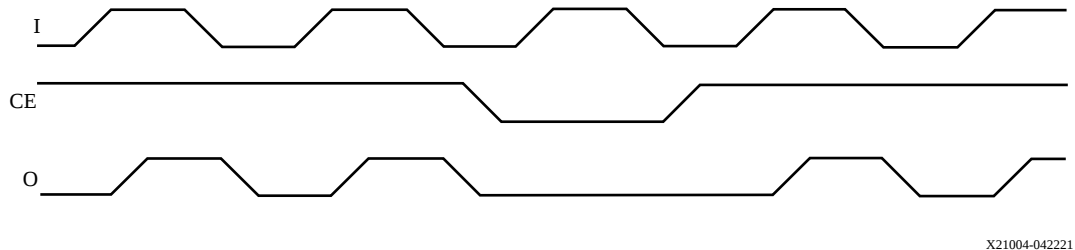
Figure 20: BUFGCE Timing Diagram
