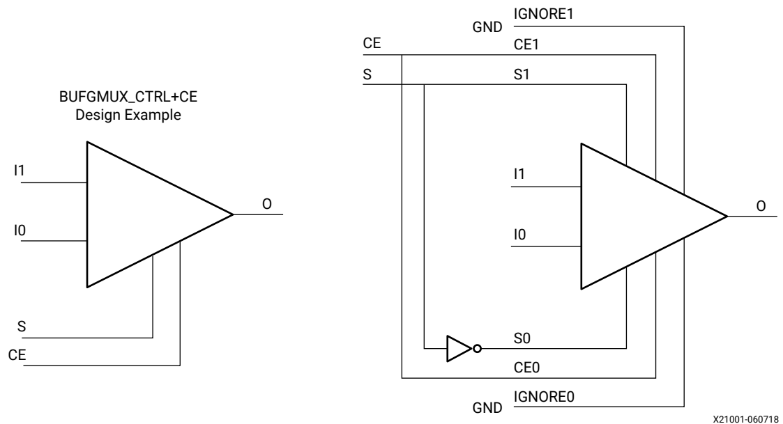
Figure 10: BUFGMUX using BUFGCTRL
