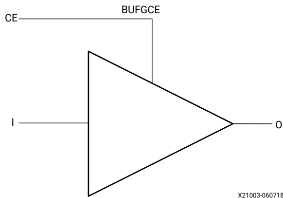
Figure 19: BUFGCE with CE
