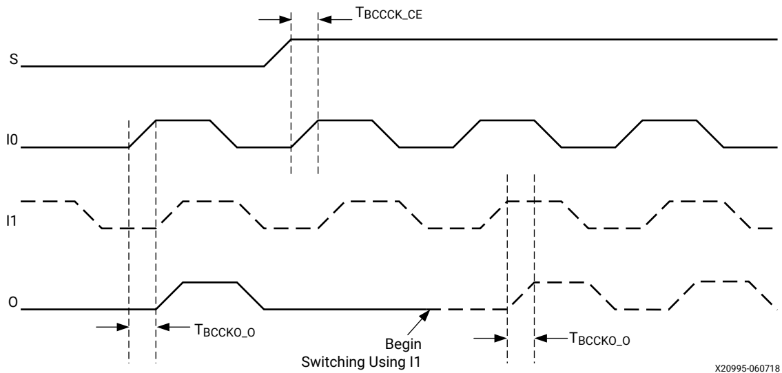
Figure 11: BUFGMUX Timing Diagram
