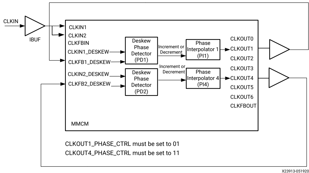
Figure 41: MMCM Deskew using PDs Connections and CLKOUTn_PHASE_CTRL Settings
