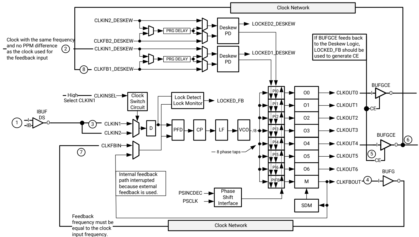
Figure 40: Example of an MMCM Using DESKEW for a Single Clock Output
