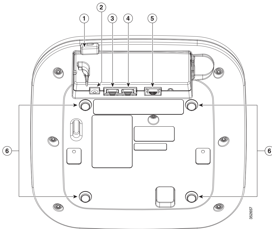
Figure 2 Access Point Ports and Connections (bottom)-AIR1702I Model
