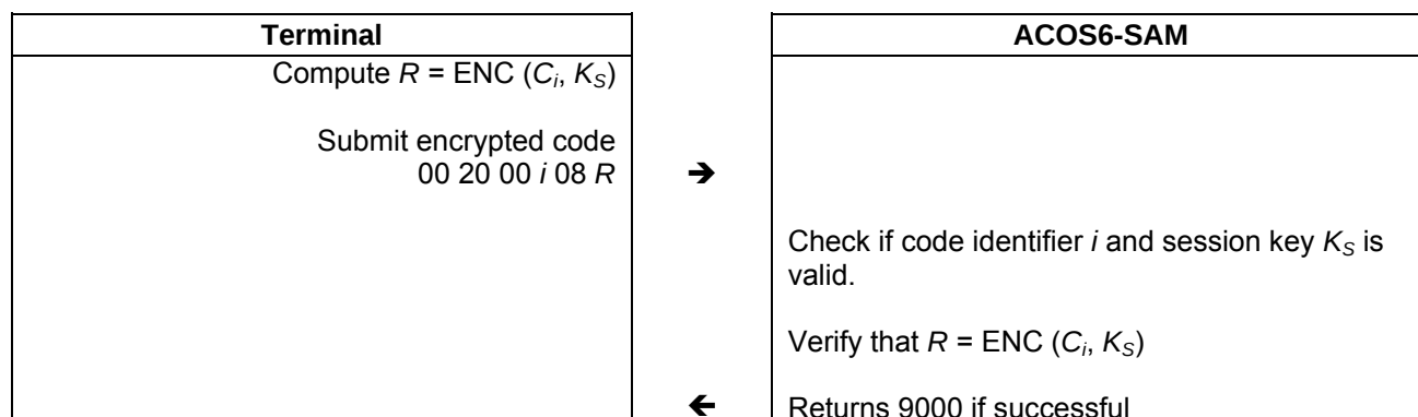
Figure 12: Submit encrypted code procedure
