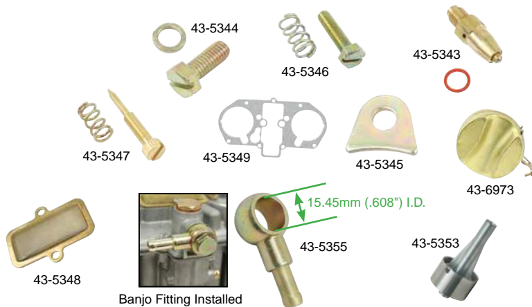
Banjo Fitting Installed
