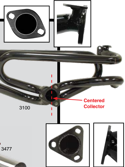
Re-Designed New Level Fit Mufflers and Collector is Centered on Header at 1:00 Position
