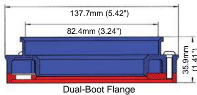
Dual-Boot Flange
