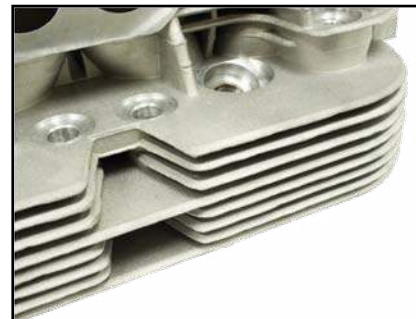
Knife-Edged Fins for Maximum Air Flow and Cooling
