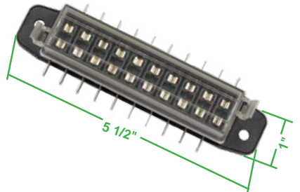
Style of Fuse
