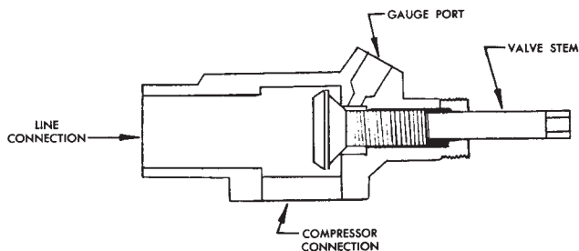
Valve Backseated
