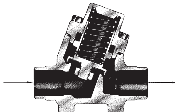
TYPICAL SPRING LOADED CHECK VALVE
