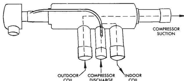
FOUR-WAY VALVE, REFRIGERANT FLOW DURING HEATING CYCLE
