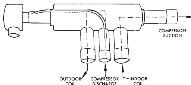
FOUR-WAY VALVE, REFRIGERANT FLOW DURING COOLING CYCLE
