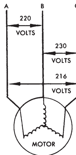
VOLTAGE UNBALANCE IN POWER SUPPLY
