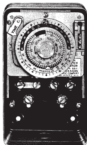
DEFROST TIME CLOCK
