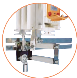
Bolted neutral link instead of direct cable connection to neutral busbar
