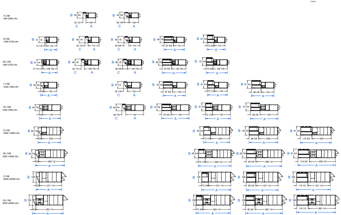
FIGURE 1 - JR SERIES CABINET LINEUP
