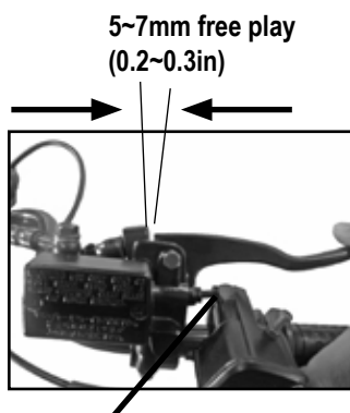
Adjustment screw
