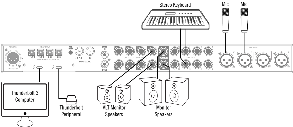
Typical Apollo x8 connections
