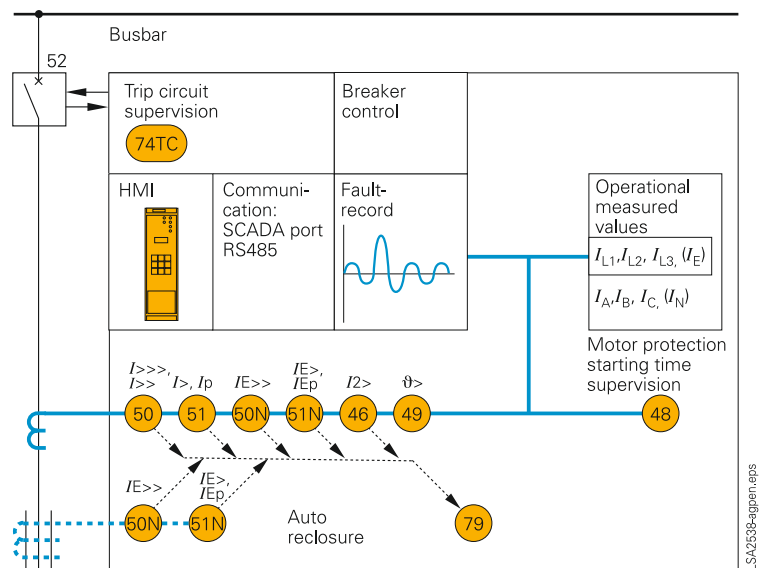
Fig. 5/20 Function diagram
