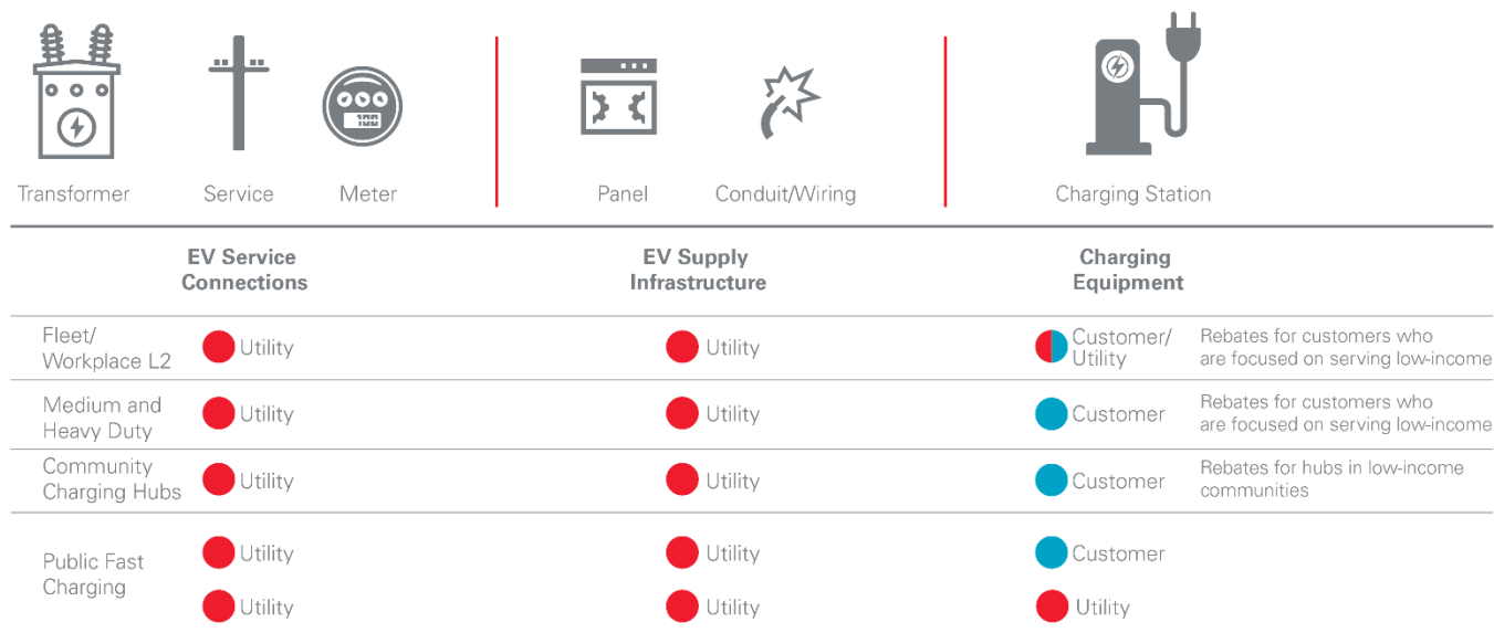
Figure 7: Infrastructure Components for Commercial Programs
