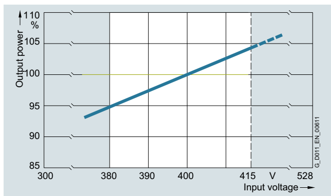
Permissible output power as a function of the input voltage for 400-V-SINAMICS G120X converters frame sizes FSA to FSG at 100% output current in the range of 380 V to 415 V (the temperature protection of the converter can reduce the current or pulse frequency above 415 V)
