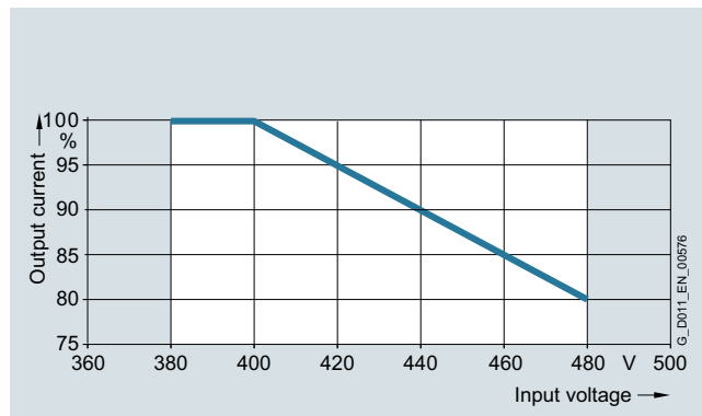
Permissible output current as a function of input voltage for 400 V SINAMICS G120X converters, frame sizes FSH and FSJ, for low overload (LO)
