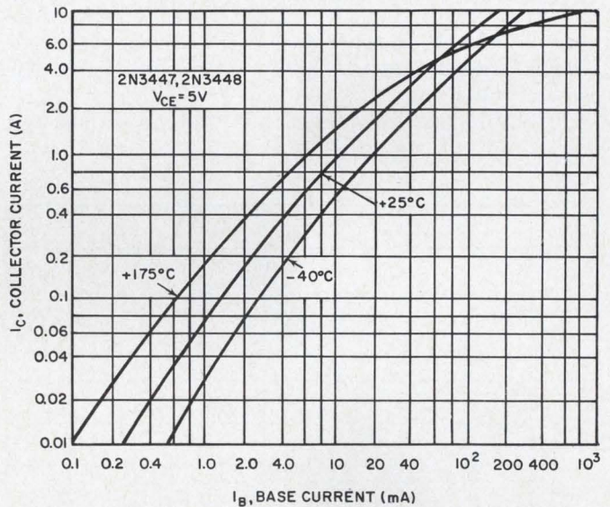
2. Collector current vs base current for a small-junction germanium unit is a function of temperature (a). The dotted line shows the I_B values at 100^\circ\text{C} with I_{CBO} included. Solid lines refer to I_B exclusively. With silicon power transistors (b) the changes in current gain are greater, although a wider ambient range is tolerated.
