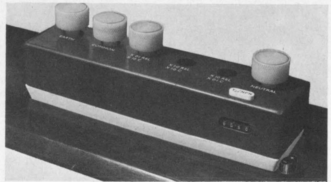
5. Adapter for WK601 unit measures just y_{21} parameter for npn transistor. Other adapters are available for other parameter measurements. Note the in-line socket arrangement which requires a socket adapter to mount transistor.
