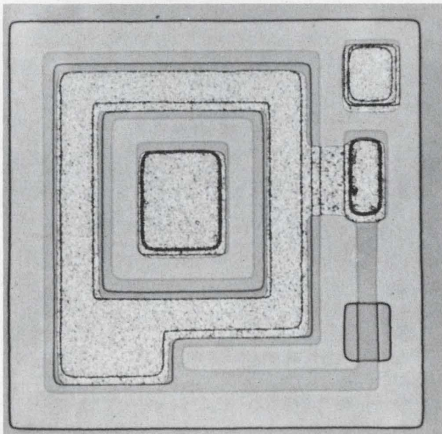
Gem of a trigger —SUS pellet geometry is used to explain functioning facets. Small contact in center is anode p-region; substrate is n material. Peripheral pn diffusions form the npn base-emitter junction; contact is made to the n region to form the cathode (see Fig. 1). The small p-channel running along the outside with a heavy n-diffusion overlay form the buried resistor R_B .
