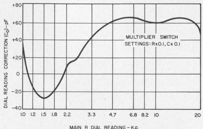
6. Each individual WK601 requires a correction curve, which must be added to all calculations to obtain correct answers.
