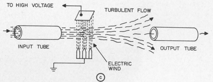
4. In the turbulence amplifier (a and b) there is an output only if no control flow turns the laminar main stream turbulent. This NOR element, made by the Howie Corp., Norristown, Pa., can be used as a building block to make other logic functions. M.I.T. has worked on the electrophoretic method of making a laminar flow turbulent (c).
