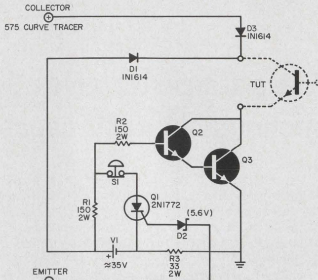
575 CURVE TRACER Circuit tests second-breakdown of transistors without any danger of device damage. Transistor Q2 and Q3 absorb excess test energy; TUT refers to transistor under test.
