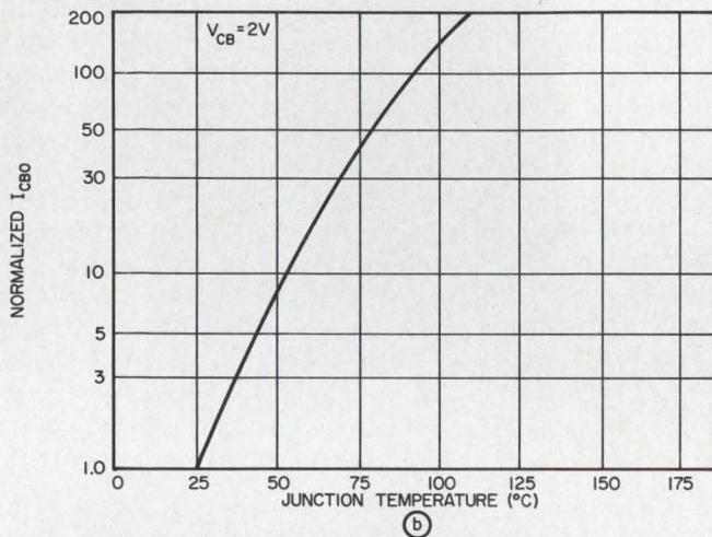
1. Changes in I_{CBO} with junction temperature for a number of different power transistors is evident (a). Ge here refers to germanium types; Si to silicon units. Measurements were made with a voltage of one-half the BV_{CEO} rating and with V_{CB} = 2 volts. The dotted curve [ I_{CBO} (2)^{\Delta T/10} ] refers to leakage doubling for every 10^\circ\text{C} increase in temperature, and serves as a comparison standard. The plot of normalized I_{CBO} vs junction temperature (b) may then be used to predict I_{CBO} variation in germanium units.
