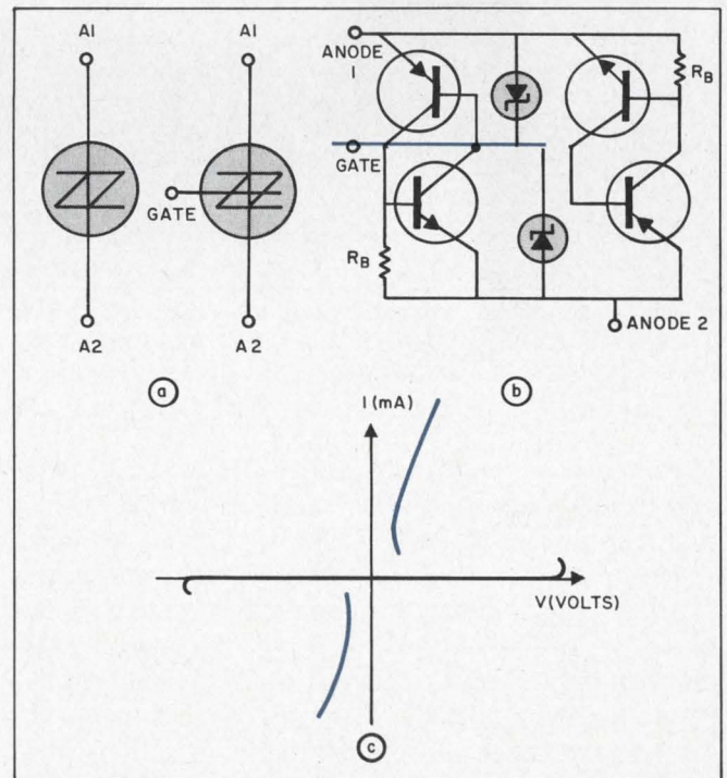
2. Silicon bilateral switch (SBS) is two SUSs connected in parallel opposition (a). Equivalent circuit (b) shows common gate lead. V-I characteristic (c) exhibits symmetry between forward and reverse directions.
