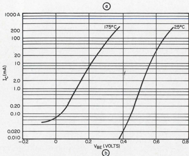
3. Transconductance vs temperature plot shows how V_{BE} changes in temperature affect biasing (a). Dotted lines refer to a V_{CE} value of 25 volts (transistor in OFF state) and solid lines are for V_{CE} = 2 volts (ON state). With a silicon power device (2N3447) operating at V_{CE} = 50 V (b), the \Delta V_{BE} rate is 2.2 mV/°C between 25 and 175°C.
