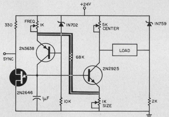
UJT added to high-impedance amplifier in a dc-bootstrapped configuration and feedback arrangement provide circuit with a linear, variable-output capability.
