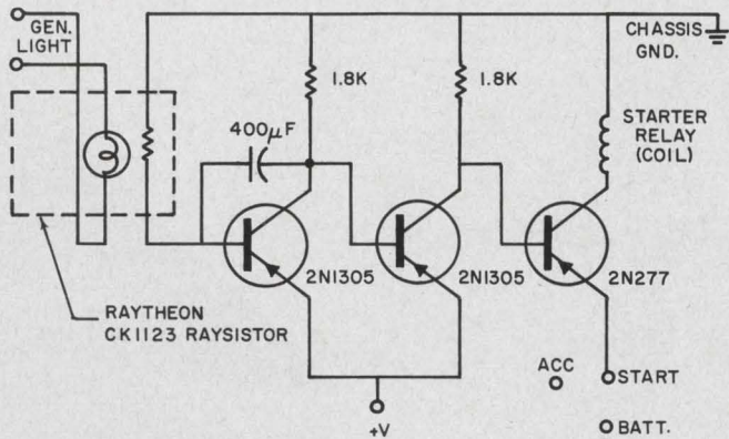
Auto-starter protection network consists of Raysistor and three bipolar stages. Starter relay is isolated from "double-start" inducers.
