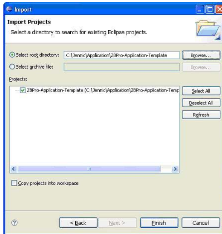
Figure 23: Import Project
