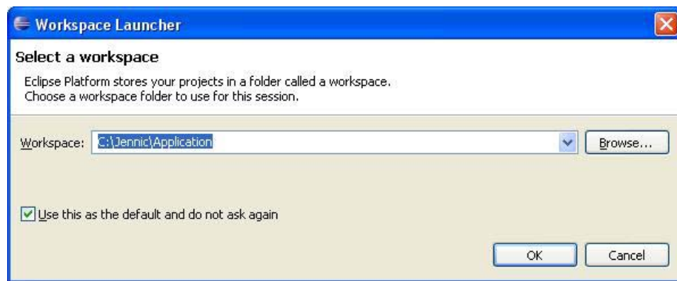
Figure 10: Workspace Launcher
