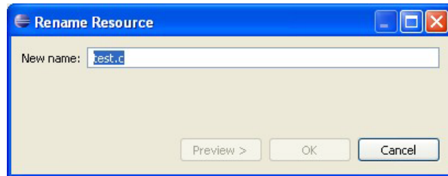
Figure 25: Rename Resource
