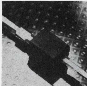
Low-cost varactor diodes with high Q, linear response and a spread of 5 to 1 at 3 to 30 v are for use in solid state tv tuners, instrumentation, and microwave circuits. The completely passivated devices provide superior mechanical shock resistance through solid junction-to-lead construction. Kollstan Semiconductors, 111 New York Ave., Westbury, N.Y. [440]
