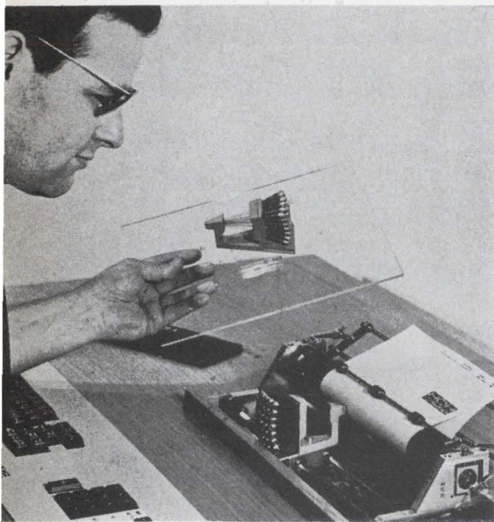
Type cast. An array of solenoids at one end of type head push pins at other end to generate characters.
