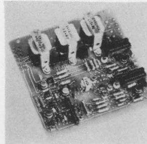
Synchro-to-sine/cosine converter series 421 features automatic voltage compensation. It will accept the output of a standard three-wire synchro and provide two isolated d-c voltages: one corresponding to the sine of the rotor shaft angle, and one corresponding to the cosine. Price is about $400-$450. Natel Engineering Co., 8944 Mason Ave., Canoga Park, Calif. [383]
