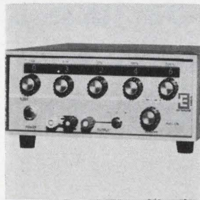
Variable d-c voltage standard model V-2000 features 1 \mu v resolution and 0.005% accuracy. Output range is up to \pm 11.1110 v in 5 decades. Front-mounted rotary switches control illuminated readout. A \pm 1 mv vernier switch aids range control. Output current of 50 ma increases versatility. Price is $625. Esterline Angus Division of Esterline Corp., Box 24000, Indianapolis 46224 [367]
