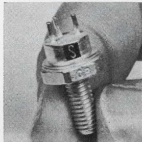
R-f power transistor type 2N5016 is a silicon npn interdigitated device. It is capable of 15 w output power at an operating frequency of 400 Mhz. It can dissipate 30 w at case temperature of up to 50^\circ\text{C} and has a saturated output power of 21 w. Price is $35.10 each in quantities of 1 to 99. Solitron Devices Inc., 1177 Blue Heron Blvd., Riviera Beach, Fla. 33404 [441]
