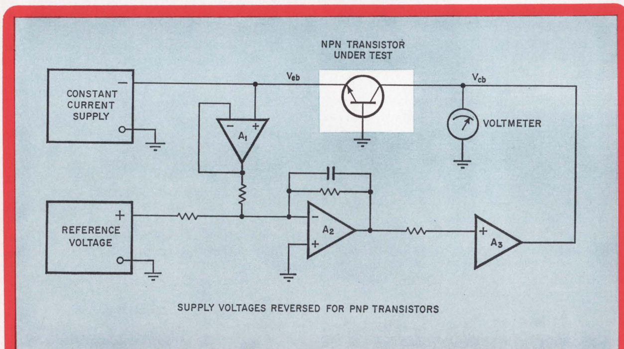
Measuring up. The transistor is immersed in two different temperature baths while maintaining a constant emitter current. The feedback circuit senses changes in V_{eb} from the reference voltage, driving V_{eb} so that it increases the collector-base junction temperature. This, in turn, drives V_{eb} back to nominal value.
