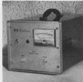
Power amplifier model 310L can provide over 10 watts of r-f power output from 250 khz to 110 Mhz. Its flat 50 db gain permits it to be driven to its full power output by all signal and sweep generators. Applications are in antenna testing, transmitter design, laser modulation and rfi/emf testing. Electronic Navigation Industries Inc., Main St. East, Rochester, N.Y. [387]
