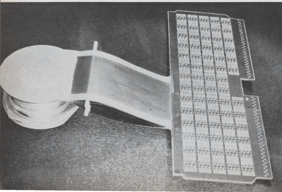
Interconnector. Rigid for mounting rows of small connectors, this integral cable multilayer board has unbonded cable extensions that remain flexible to round connector, where they are bonded and rigidized.
