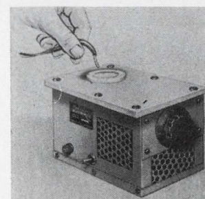
High-temperature (in excess of 1,300°F) silver soldering pot eliminates need for chemical or abrasive removal of film insulation and use of soft solder and soldering iron when joining magnet wires to leads. Dipping wires into molten solder simultaneously strips insulation and encases them in a permanent silver solder coating. Precision Electronics Corp., Marshfield, Mass. [428]
