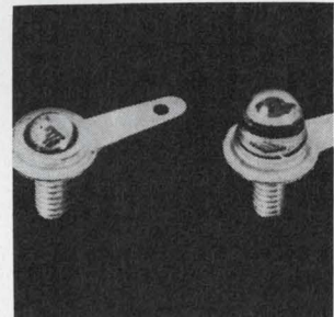
High-power light-emitting diodes series ME2 and ME5 are large area, gallium arsenide units with spectral emissions in the near infrared range peaking at 9,000 angstroms. At 1 ampere continuous input current they have a total radiated minimum output power of 10 mw from a 50-x-50-mil emitting area. Monsanto Electronic Special Products, 10131 Bubb Rd., Cupertino, Calif. [439]
