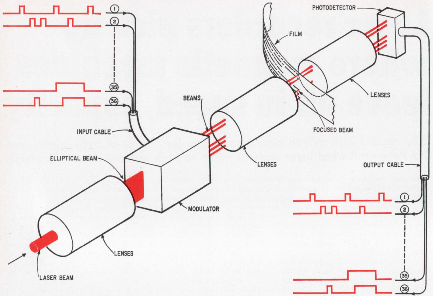
Bits onto film. Driven by the recorder's 36 input signals, the modulator converts a single laser beam into 36 information-carrying beams, which are focused onto the film.
