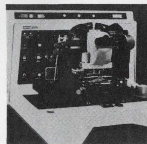
Fully automatic mask alignment system called Autolign 2686 is designed for integrated circuit production. It accommodates wafers up to 3 in. in diameter and positions mask-to-wafer with an accuracy of better than 1 micron. Typical alignment time is 4 to 6 seconds versus the conventional 20 to 30 seconds. Price is $29,750. Kulicke & Soffa Inc., Fort Washington, Pa. 19034 [424]
