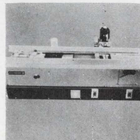
Bench type wave-soldering system model 94 is designed for fully automated production of chips, substrates, micromodules, flat-packs, or p-c boards up to 6 in. wide. It consists of a foam fluxer, preheater, soldering unit, board-holder carrier and conveyor. It operates at temperatures up to 600°F. Price is under $3,000. Electrovert Inc., 85 Hartford Ave., Mt. Vernon, N.Y. [426]
