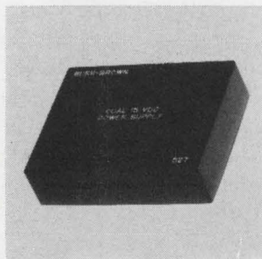
Encapsulated power supply model 527 provides two 15 v power supplies capable of common external connections with an accuracy of 1%. Each separately regulated supply provides a full 50 ma of output current. Output regulation, line or load is \pm 0.2\% . Temperature stability is \pm 0.02\% / ^\circ\text{C} . Price is $39; delivery, stock to four weeks. Burr-Brown Research Corp., Tucson [385]
