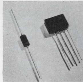
Silicon rectifier series MHR can handle 300 amp surges at 100^\circ\text{C} . Voltage ratings at 100-1,000 v piv are standard. Units meet or exceed requirements of Mil-Std-202B method 103A and all other specifications of NEMA-EIA Class A2. Prices start at 23 cents each in 1,000 lot quantities for the MHR100. Micro Semiconductor Corp., 11250 Playa Court, Culver City, Calif. 90230 [438]
