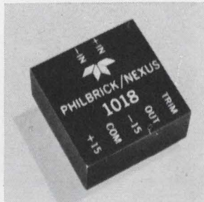
Chopperless, differential operational amplifier model 1018 features low drift. It employs dual-input transistors with a precision metal-film resistor and a bias current compensation network. This results in high thermal stability and low static offsets. Typical gain is 2,000,000; output, \pm 3.5 ma at \pm 13 v. Philbrick/Nexus Research, Allied Dr. at Route 128, Dedham, Mass. [382]
