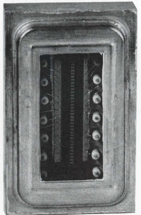
One beam; one diode. With its column of 36 GaAs diodes, the recorder's photodetector turns the incoming beams into 15-mv outputs.
