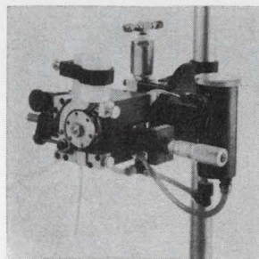
Designed for the automated dispensing of 500 micrograms to 500 milligrams of reactive resins and chemicals, the Picoshot adapter is for precision bonding, potting, and junction coating in the semiconductor and components industry, and for precision application of adhesive products in assembly operations. Fluidyne Instrumentation, Mt. Diablo Blvd., Lafayette, Calif. [423]
