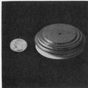
Silicon controlled rectifier called Astro-Pack, with a 48-mm pellet diameter, can supply up to 1,500 amps and up to 1,200 v. It offers 1^2\text{T} up to 1 million. It supplies up to 2,000 amps rms in an a-c switch in a water cooled configuration. Applications include motor controls and electromechanical power supplies. Power Semiconductors Inc., 90 Munson St., Devon, Conn. 06460 [442]
