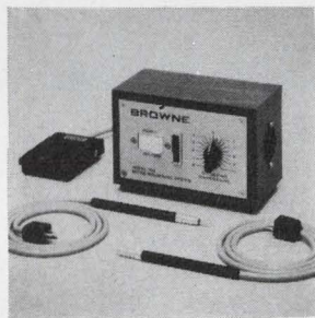
Autopulse soldering system model 150 is for delicate hybrid IC soldering processes. It is supplied complete with a stepless variac power supply, foot switch actuator, micro-loop hand probe, microgap tungsten resistance hand probe, and a full assortment of replacement tip elements. Price is $175. Browne Engineering Co., Coast Village Circle, Santa Barbara, Calif. [422]
