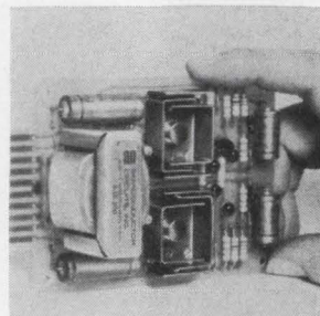
Plug-in power supplies series J feature an isolation factor of 10,000 megohms with 1 pf maximum capacitance. They are for use with medical instruments, machine tool controls, strain gauge bridges, and transducers. Series includes both single and dual d-c outputs at 10, 12, and 15 v and 50, 100 and 200 ma. Semiconductor Circuits Inc., Merimac St., Woburn, Mass. [388]
