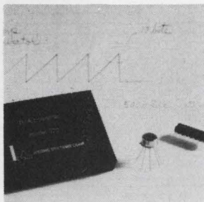
D/A converter model 320 contains a complete set of switches and a resistance ladder. Full scale output is 15 ma which may be converted to a voltage by means of a resistor to ground. The unit's fast settling of 750 nsec for 10 bits and 200 nsec for 8 bits makes it suitable for use in graphic display systems. Hybrid Systems Corp., 95 Terrace Hall Ave., Burlington, Mass. 01803 [381]
