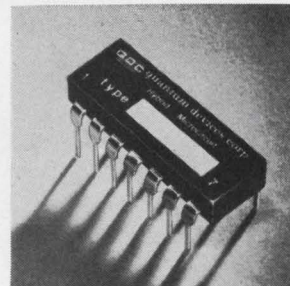
Operational amplifier OA201 features a 150-ma output at 10 v. Packaged in dual in-line configuration it is also available as a hermetically sealed unit. The amplifier is short circuit proof. It operates at a very low input bias current, 200 na. Offset voltage is 25 \mu\text{v}/^\circ\text{C} , and open loop gain is greater than 100,000. Quantum Devices, 15 W. Main St., Bergenfield, N.J. [384]
