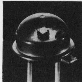
Gallium arsenide i-r emitting diode FLD 100 is suited for use in conjunction with silicon photo sensors since their spectral peaks are closely matched. Forward voltage is 1.35 v; reverse voltage, 8.3 v; wavelength at peak, 9,000 angstroms; angle between half intensity points and peak axis, 65^\circ . Fairchild Microwave and Optoelectronics, 2513 Charleston Rd., Mtn. View, Calif. [437]
