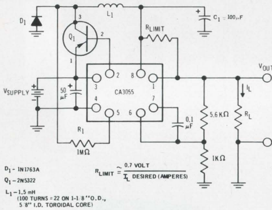
SWITCHING REGULATOR USING RCA-CA3055
