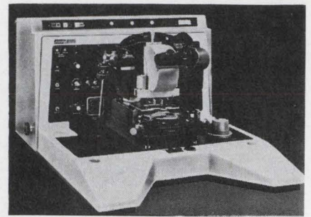
Arranger. Instrument aligns mask and wafer for manufacture of IC's
