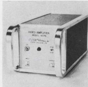
High input impedance, wideband video amplifier 4376 offers high gain and low equivalent input noise. It is useful for amplifying signals from high impedance sources and for increasing the sensitivity of lab instruments such as a wideband oscilloscope or an r-f voltmeter. It features built-in protection circuitry. Price is $395. C-Cor Electronics Inc., State College, Pa. [386]
