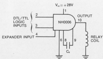
RELAY DRIVER
