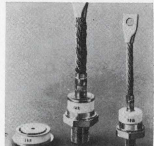
Fast recovery 100-ampere rectifiers series 101KL and 101KLR come in a DO-8 Rock-top package. Reverse recovery times are 1.5 \mu\text{sec} and 2 \mu\text{sec} with up to 100 amps at voltages from 400 to 1,300 v. Applications include inverters, phase-controlled SCR assemblies, and other areas requiring h-f fast recovery rectification. International Rectifier, El Segundo, Calif. [443]
