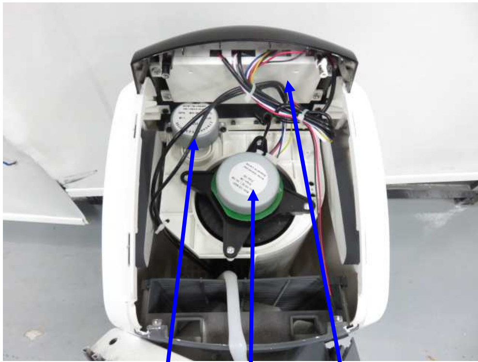
Inner view (sync. Motor, DC fan motor and main board location)
