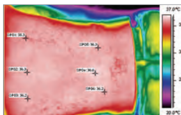
PerfectTemp Warming System. Thermal imaging shows uniform warming over a large surface area.
