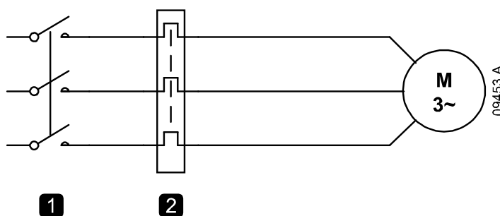
DOL starter installation
