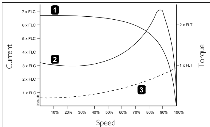
Current and torque profile for DOL starting
