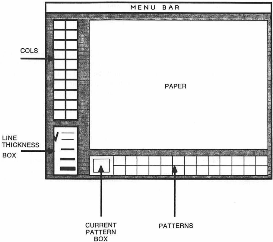
Figure 5.1 MacPaint's Components.
