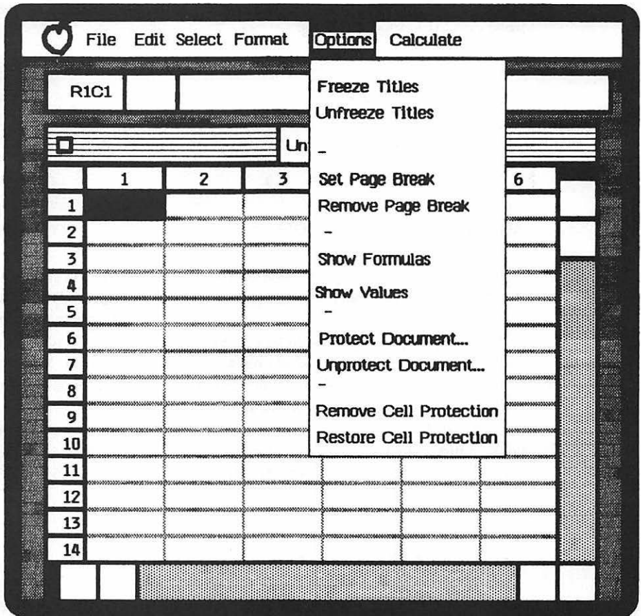
Figure 2.5 Options Menu.
