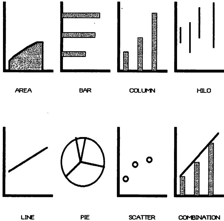
FIGURE 4.6 MACCHART SHAPES.
