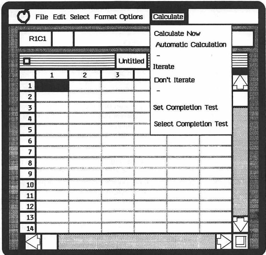
Figure 2.6 Calculate Menu.
