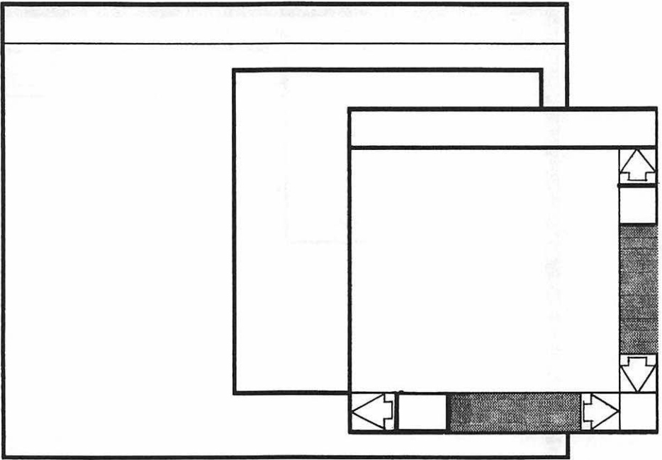
Figure 1.10 Multiple Windows.
