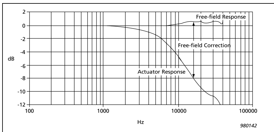
Fig. 1. Free-field Frequency Response of a Brüel & Kjær Type 4191 microphone obtained by adding the free-field correction to an individually measured Actuator Response
