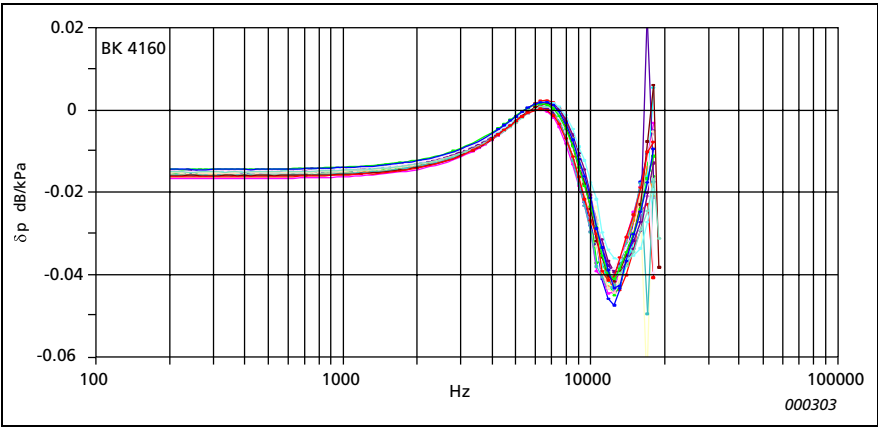
Fig. 1. Measured modulus of static pressure coefficient of 18 microphones Type Brüel & Kjær 4160
