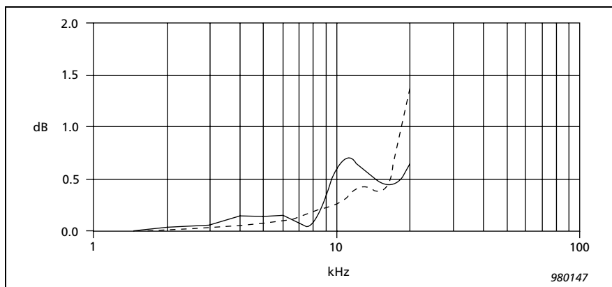
Fig. 7. Difference in free-field correction for 6 different 1/2" Brüel & Kjær Falcon Range microphones with exactly the same mechanical configuration around the diaphragm ---- Boundary Element Calculation — Brüel & Kjær measurements
