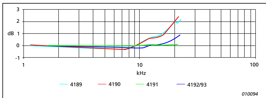
Fig. 1. Pressure-field corrections for Brüel & Kjær Falcon Range \frac{1}{2} " microphones based on pressure-field reciprocity measurements
