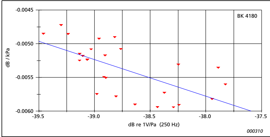
Fig. 8. Low frequency value a_0 of static pressure coefficient \delta_p as function of the pressure sensitivity level at 250 Hz for 30 Brüel & Kjær microphones Type 4180
