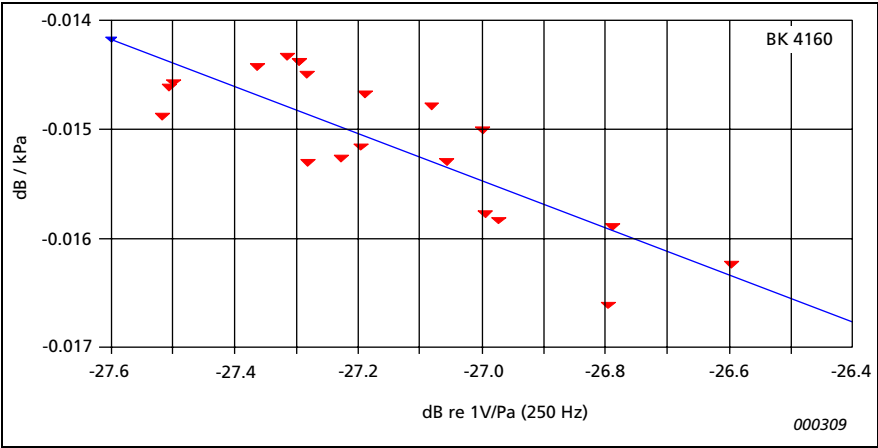
Fig. 7. Low frequency value a_0 of static pressure coefficient \delta_p as function of the pressure sensitivity level at 250 Hz for 18 microphones Brüel & Kjær Type 4160
