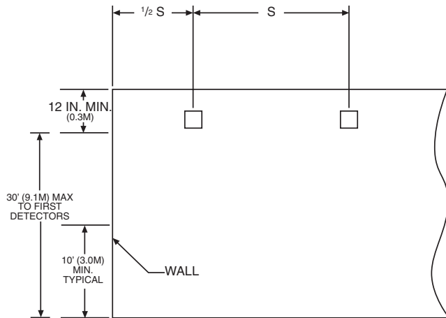
FIGURE 2. SPACING FOR SMOOTH CEILING (TOP VIEW):
