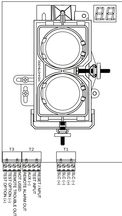
FIGURE 7. WIRING DIAGRAM
