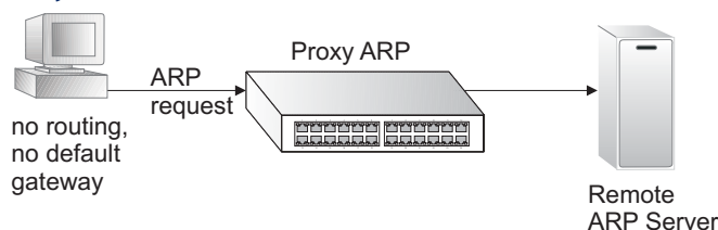
Figure 409: Proxy ARP
