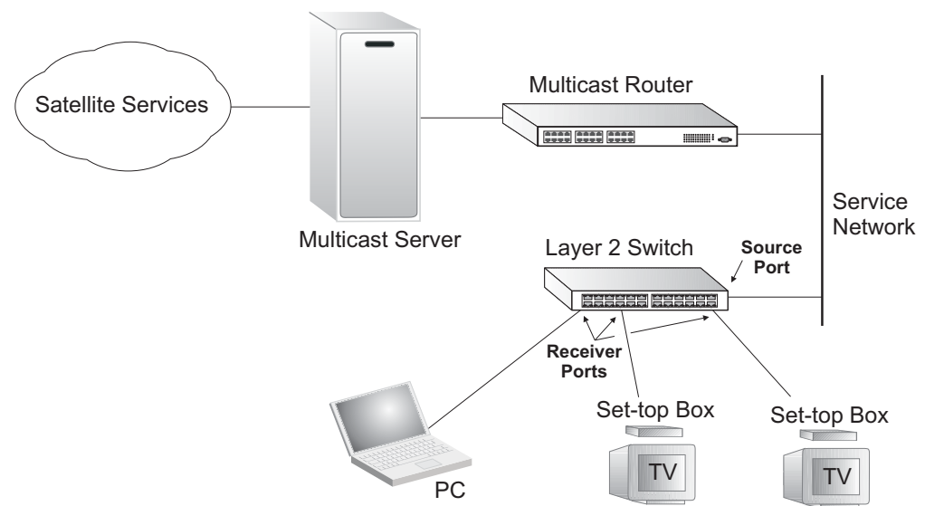
Figure 380: MVR Concept
