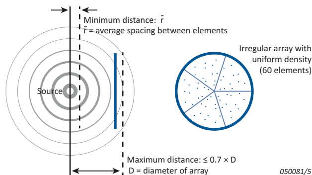
Fig. 2 Measuring distance for wideband holography
