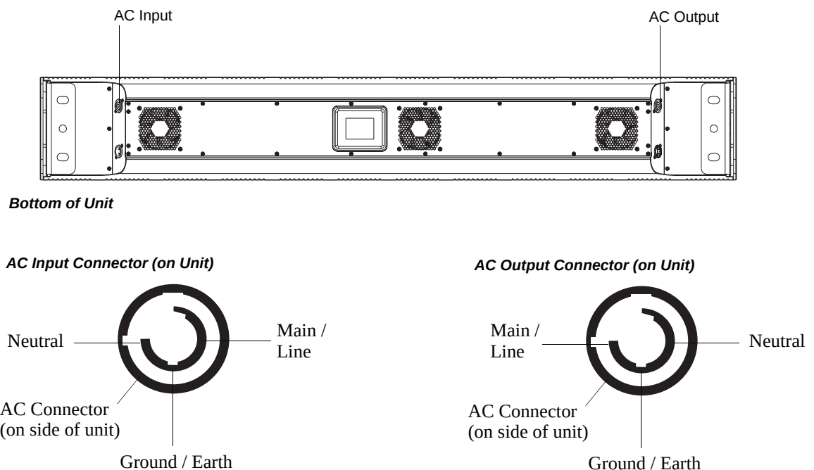
Figure 4: SL BAR 640 RGBW LED Luminaire AC Input & Output Connections
