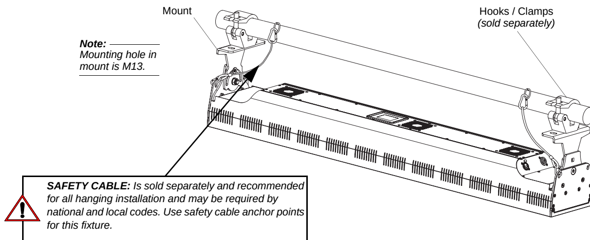
Figure 7: Mounting Luminaire - Hanging Applications
