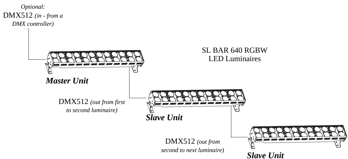
Figure 10: SL BAR 640 RGBW LED Luminaire - Master / Slave Configuration
