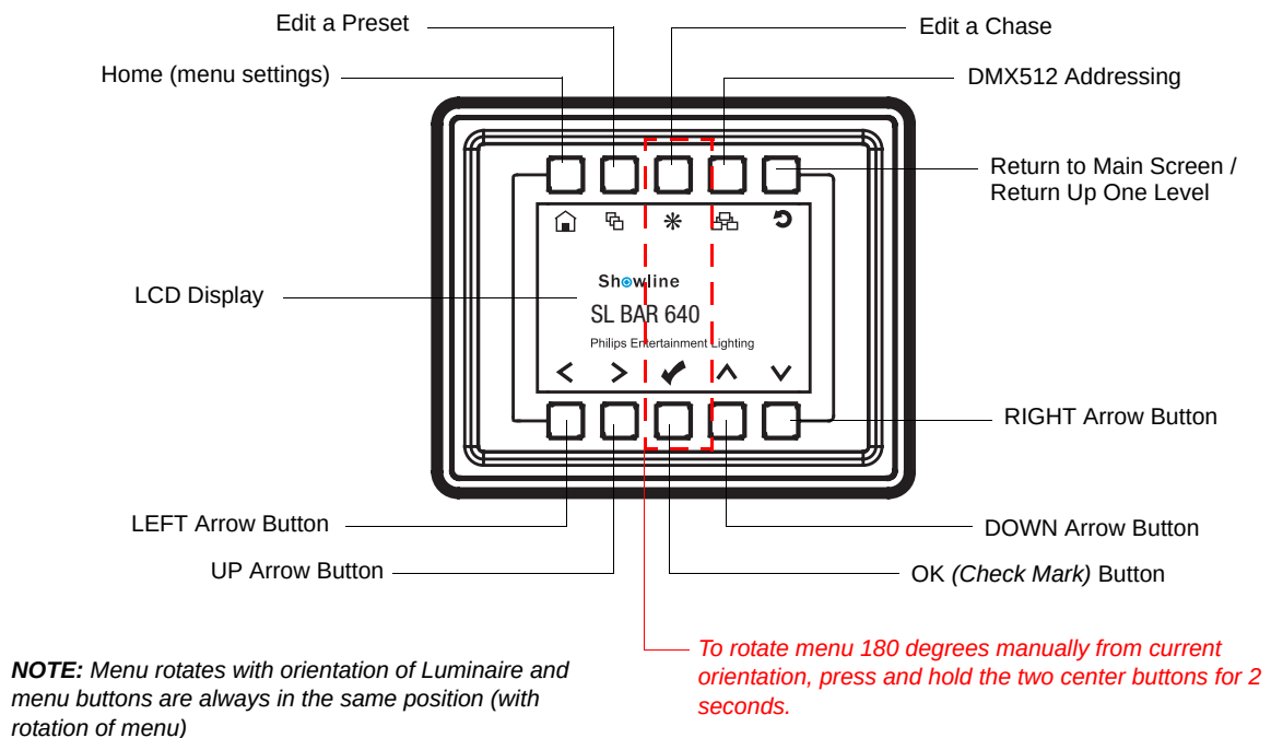
Figure 8: LCD Display and Menu System
