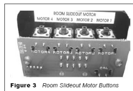
Figure 3 Room Slideout Motor Buttons
