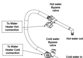
Two Valve Water Heater Bypass Valves shown in NORMAL mode
