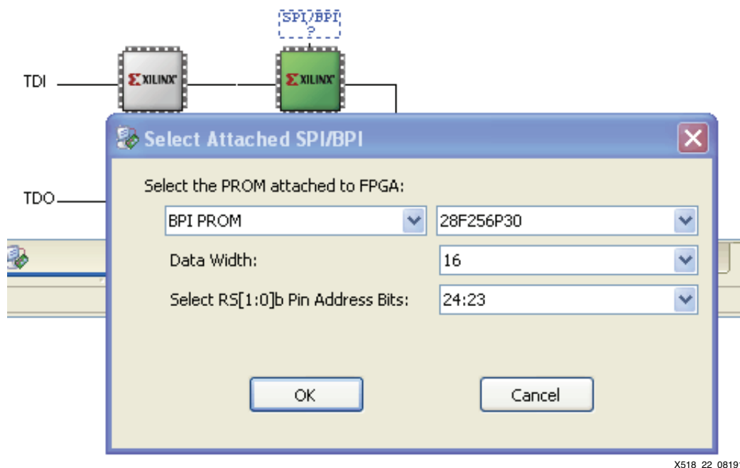
Figure 21: Set Up BPI PROM in iMPACT
