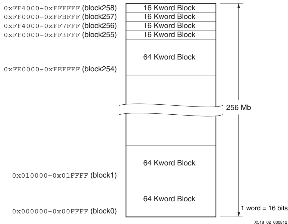
Figure 2: JS28F256P30T95 Address Map
