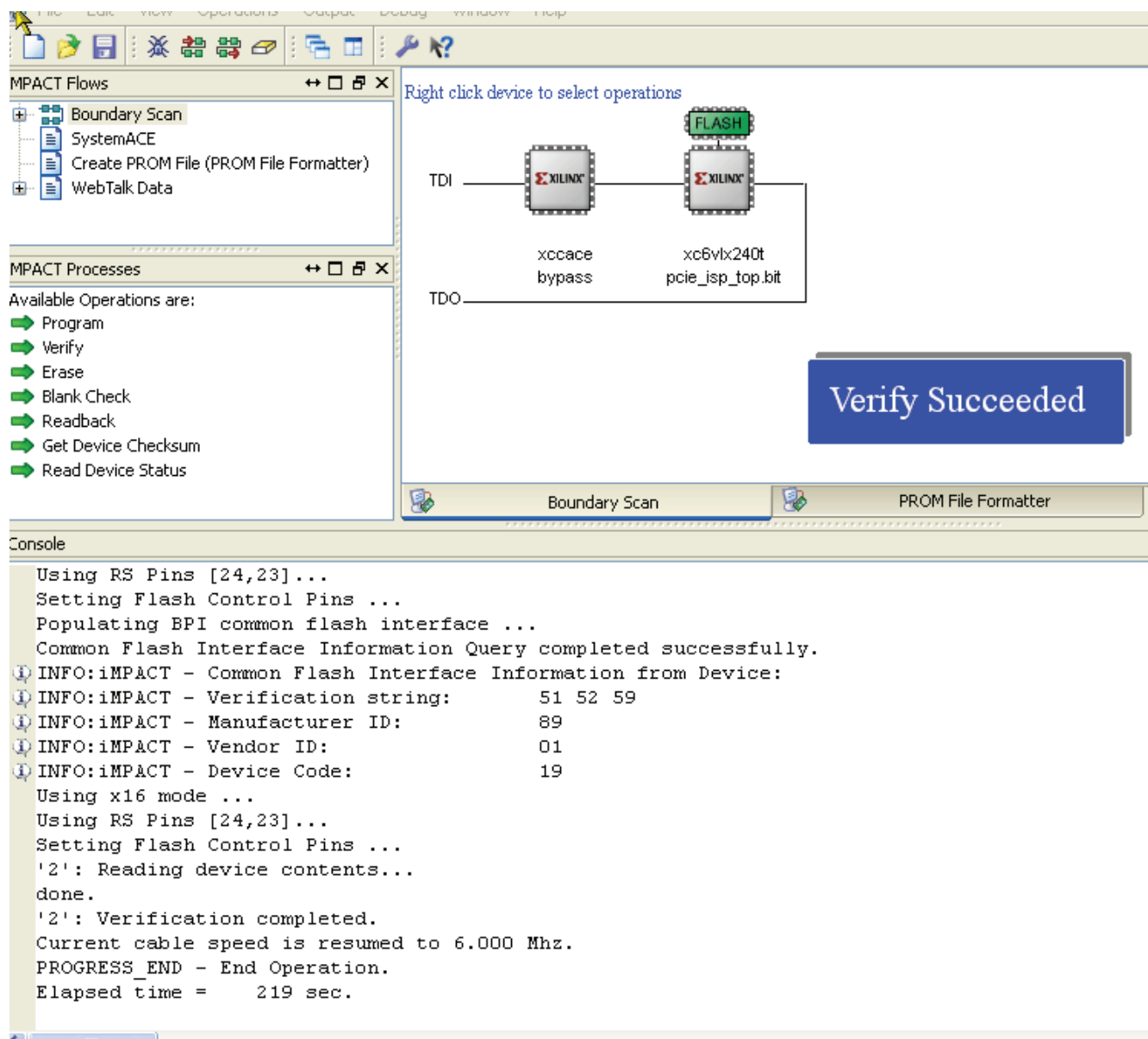
Figure 23: PROM Verification Successful
