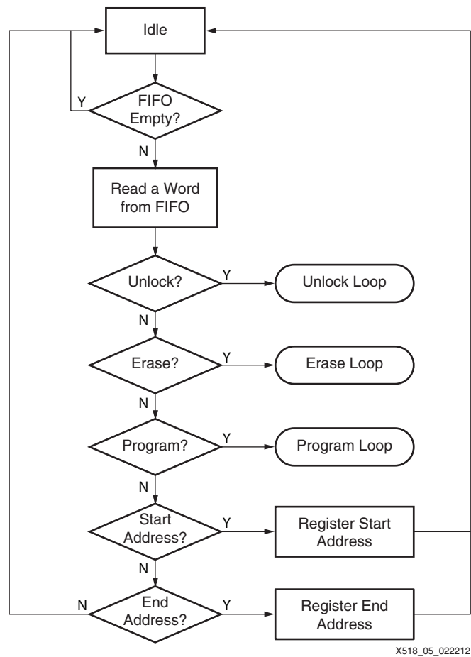
Figure 5: Main Command Loop
