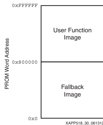
Figure 24: PROM Address Map
