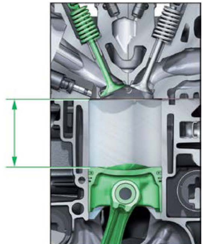
2.0T ultra engine with new B cycle combustion process
