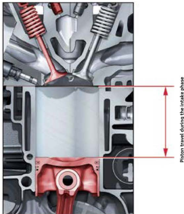
Third-generation 2.0l TFSI engine with conventional combustion process
