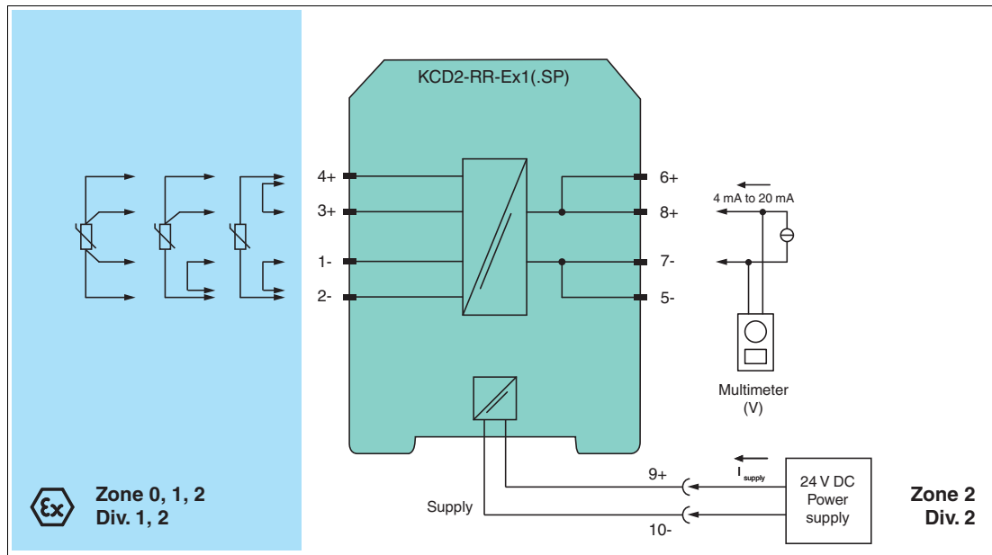
Figure 5.1 Proof test set-up for KCD2-RR2-Ex1(.SP)
