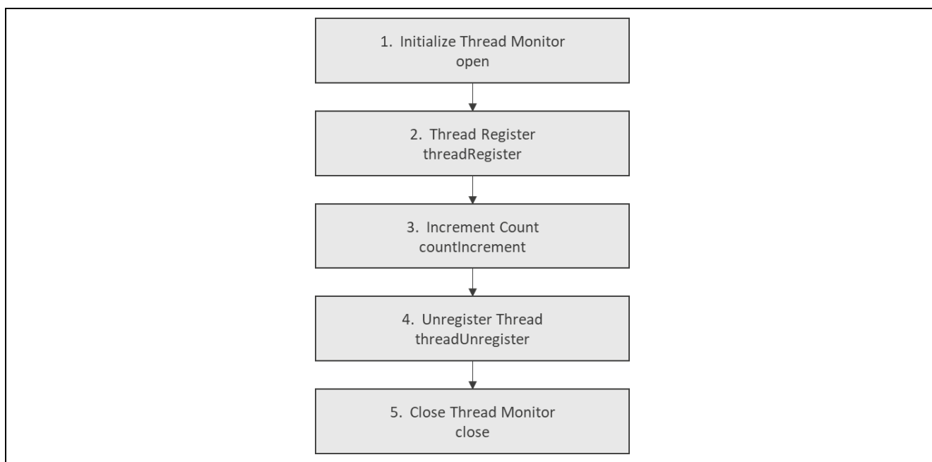
Figure 5. Typical Thread Monitor Framework Module Application
