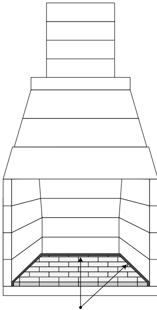
FLOOR WITH ½" EXPANSION GAP ALONG BACK AND SIDE WALLS
