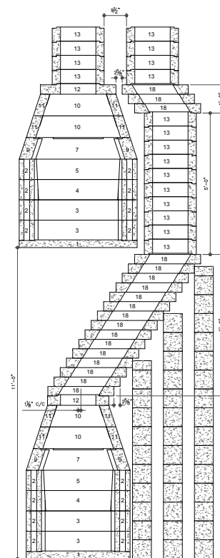
FIGURE 9.4 INSTALLATION WITH OFFSET BLOCKS (SEE FIGURE 14 ON PAGE 26 FOR MORE DETAILS)
