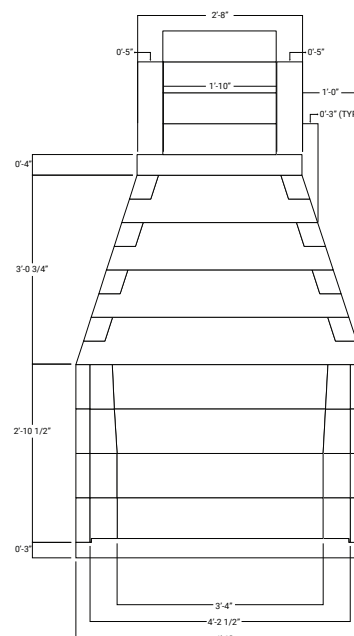
FIGURE 1.4 48" CONVENTIONAL
