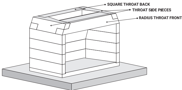
FIGURE 7.1 ASSEMBLED THROAT
