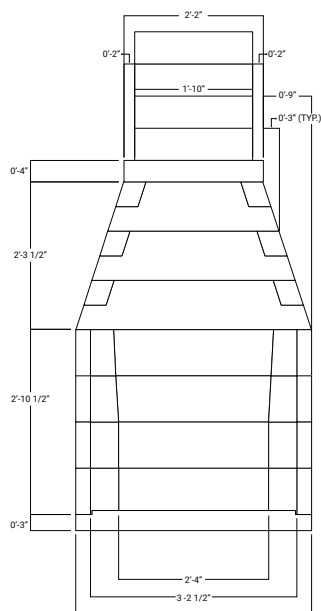
FIGURE 1.2 36" CONVENTIONAL
