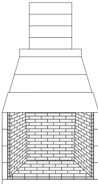
FULLY BRICKED FIREBOX COVERING EXPANSION GAPS
