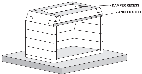
FIGURE 7.2 DAMPER RECESS + ANGLED STEEL
