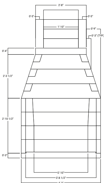
FIGURE 1.3 42" CONVENTIONAL
