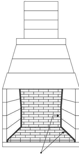
FLOOR & BACK WALL WITH ½" EXPANSION GAP ALONG SIDE WALLS
