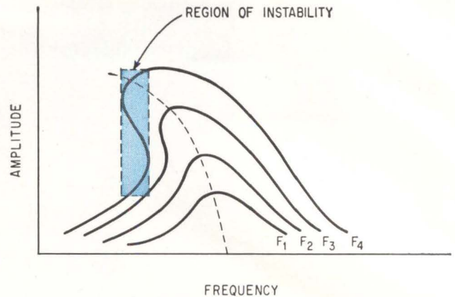
ELECTRICAL CIRCUITS containing a nonlinear reactance show a double-valued characteristic if the driving signal becomes too large—Fig. 1
