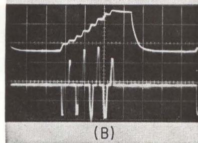
CONVENTIONAL charger waveforms, voltage, top, and current, bottom, (A); SCR charger waveforms (voltage, top, and current, bottom) provide increased efficiency due to reduced duty cycle—Fig. 3
