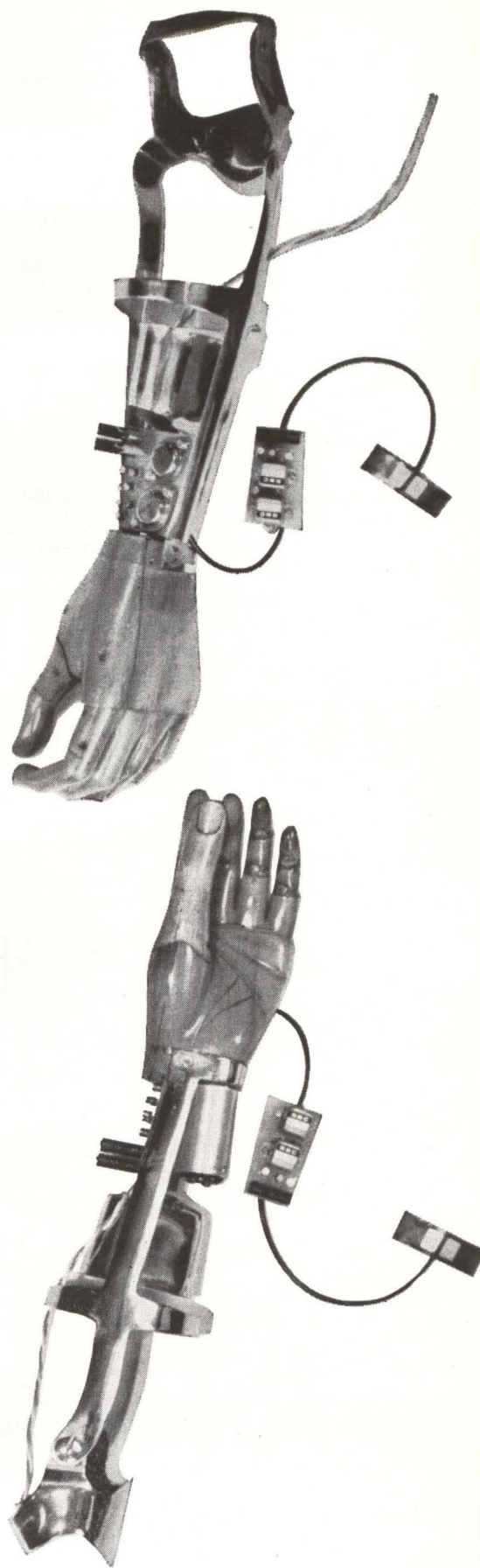
EXPOSED views of prosthetic hand with cosmetic glove and socket removed to show servoamplifier, potentiometer rotative control, and motor assembly; emg pickup electrodes are attached to adhesive strap
